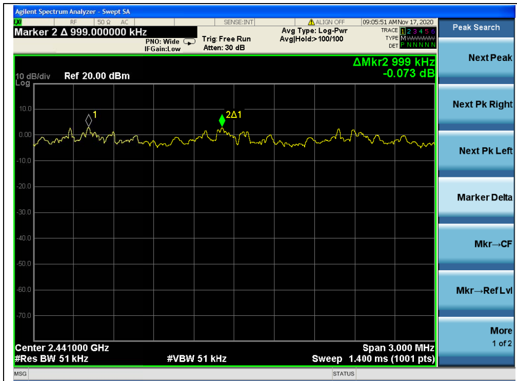
(\pi/4\text{-DQPSK})
