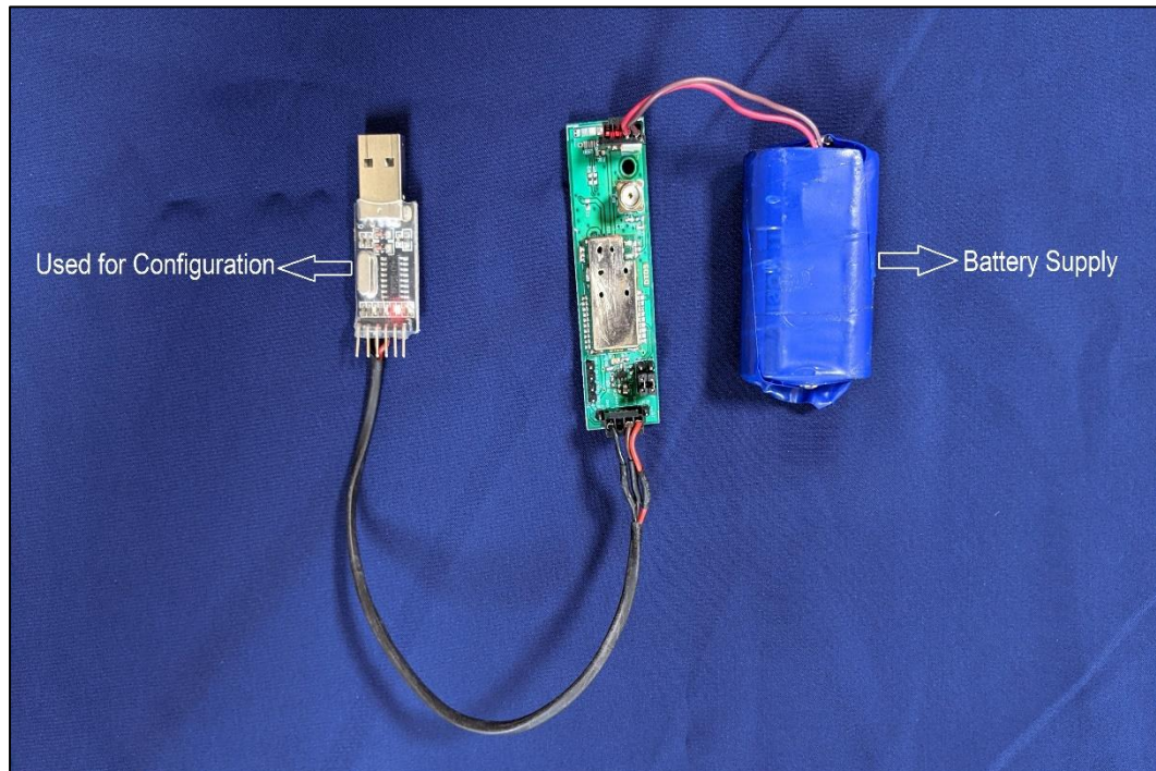
Photo 8: battery connected to Module via supporting board and USB cable used for the configuration of module via supporting board
