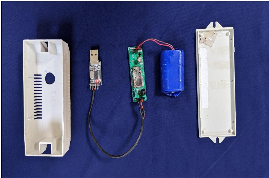
Photo 6: Plastic Enclosure Open
