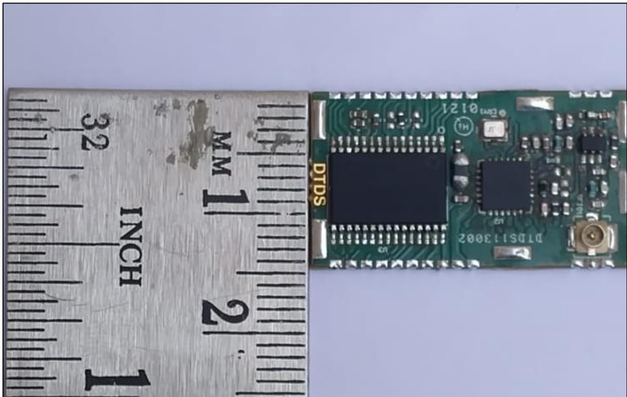
Photo 5: Module Dimensional view
