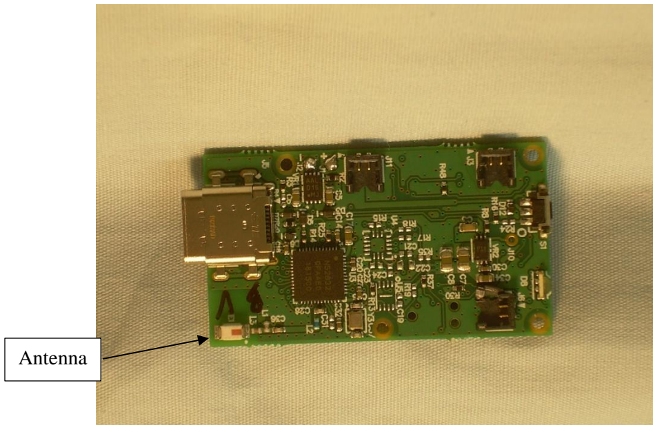
Photograph 11: View of Side A of the PCB
