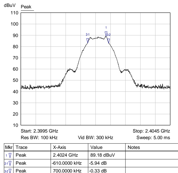
Graph 1: Lowest Channel Bandwidth
