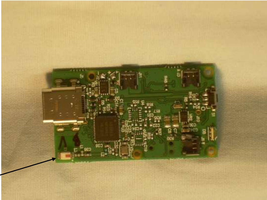
Photograph 1 – Top View of the PCB
