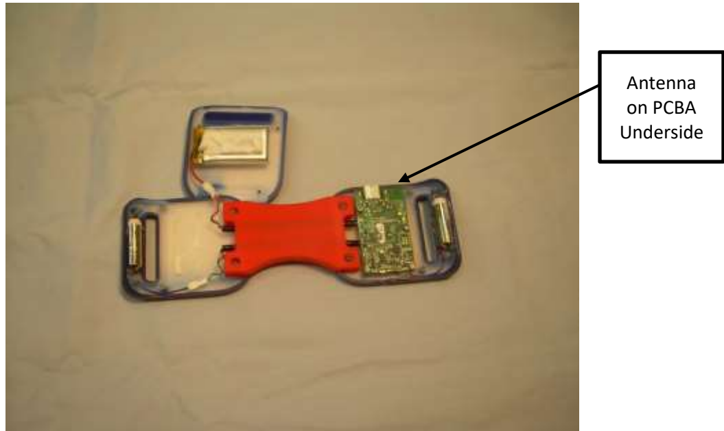
Photograph 3 – PCBA Placement View of the EUT
