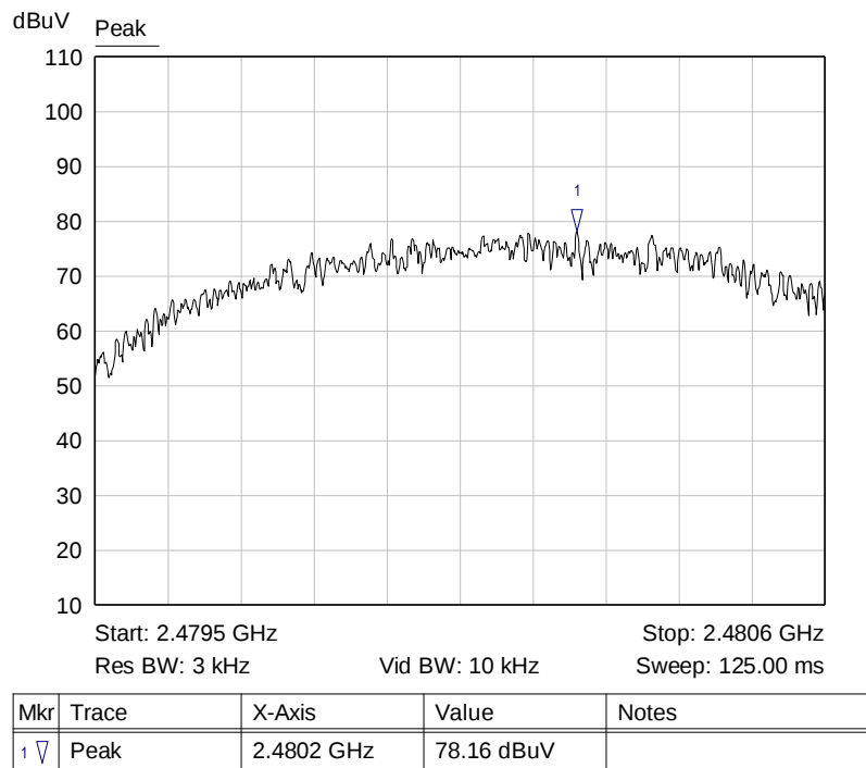
Graph 11: Highest Channel Output 3 kHz PSD Plot
