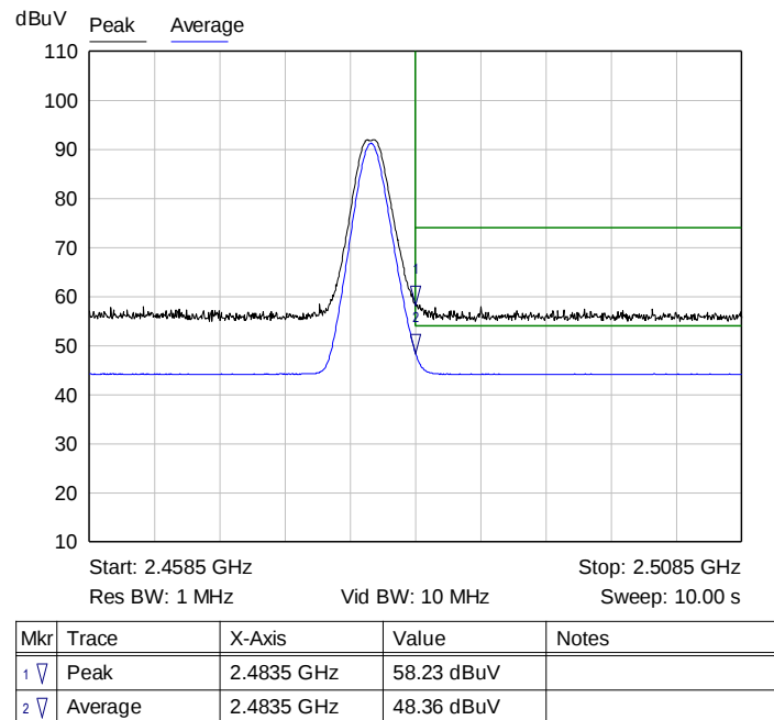
Graph 8: Radiated Upper Band Edge Plot
