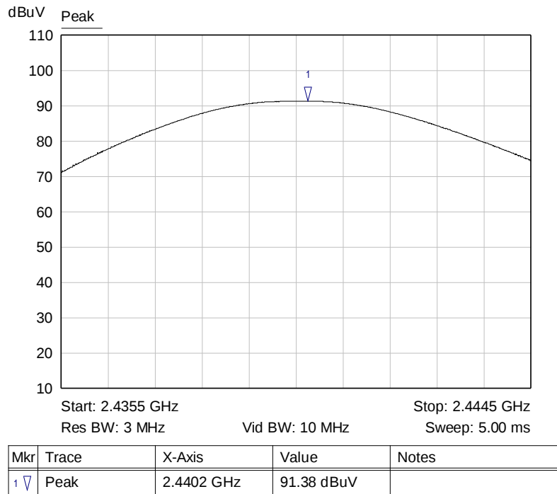
Graph 5: Middle Channel Output Power
