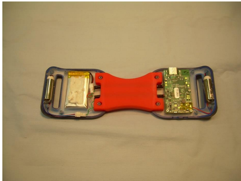
Photograph 10: View of the EUT With the Housing Opened
