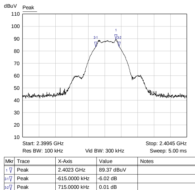
Graph 1: Lowest Channel Bandwidth
