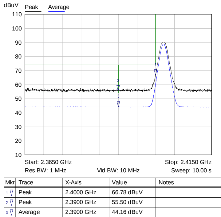
Graph 7: Radiated Lower Band Edge Plot
