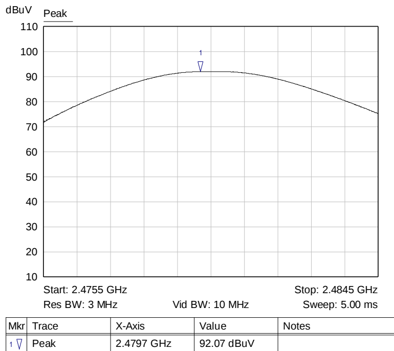
Graph 6: Highest Channel Output Power Plot
