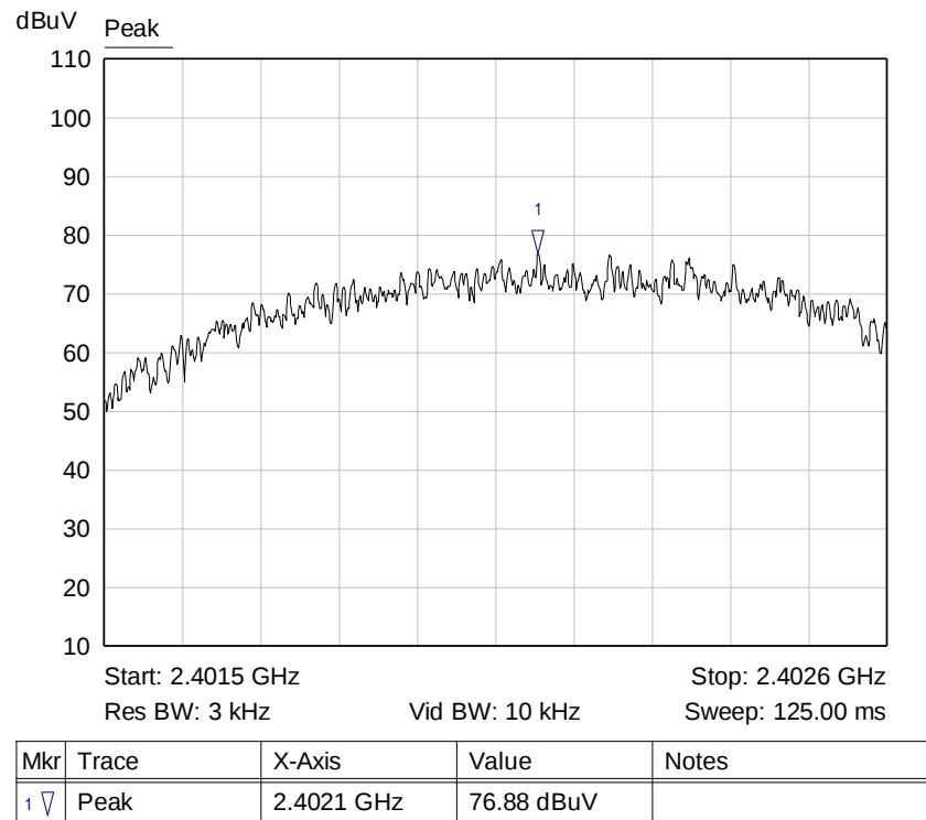
Graph 9: Lowest Channel 3 kHz PSD Plot
