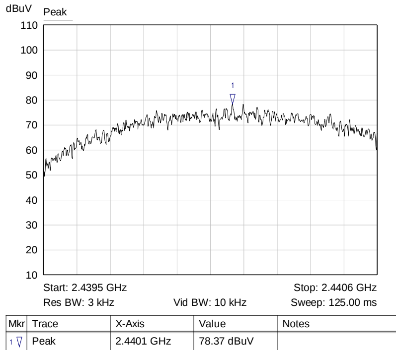
Graph 10: Middle Channel 3 kHz PSD Plot
