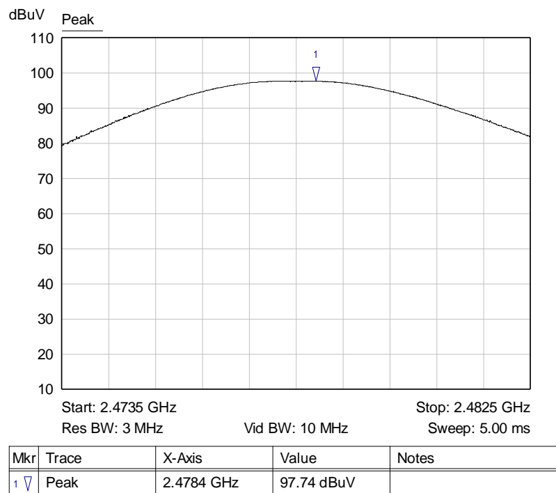
Graph 6: Highest Channel Output Power Plot
