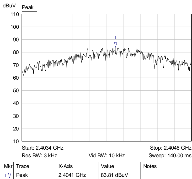
Graph 20: Lowest Channel 3 kHz PSD Plot
