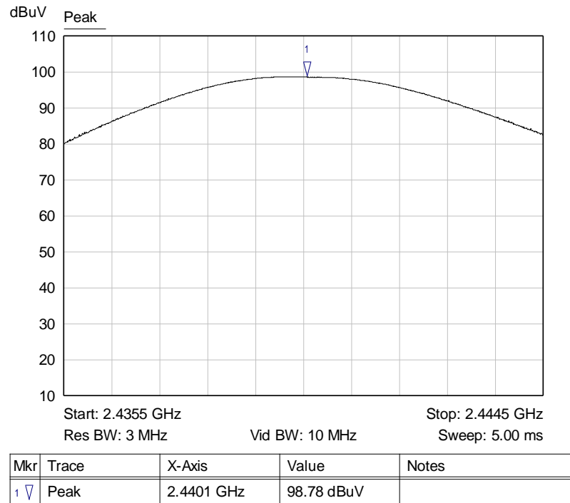
Graph 5: Middle Channel Output Power
