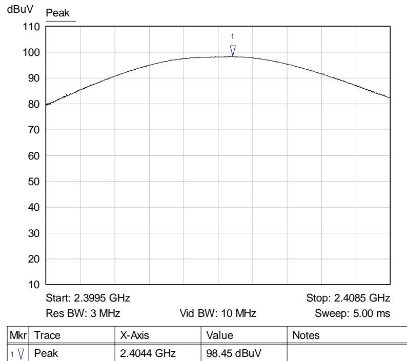
Graph 15: Lowest Channel Output Power Plot
