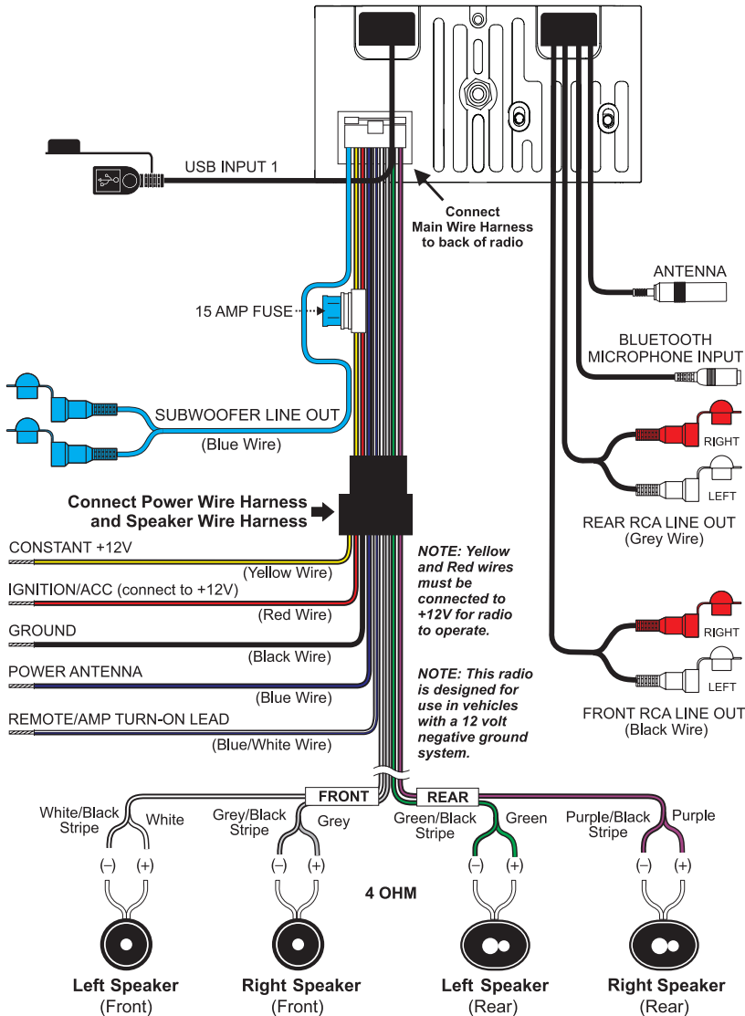
Figure 5 - Wiring Diagram
