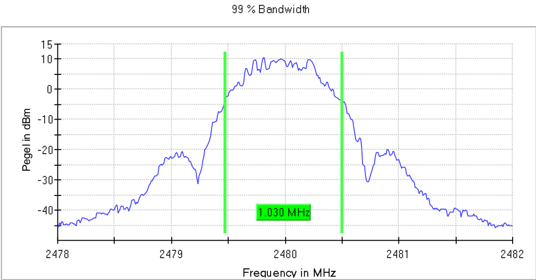
Transmission on 2480 MHz; + 85°C, 24 V DC
