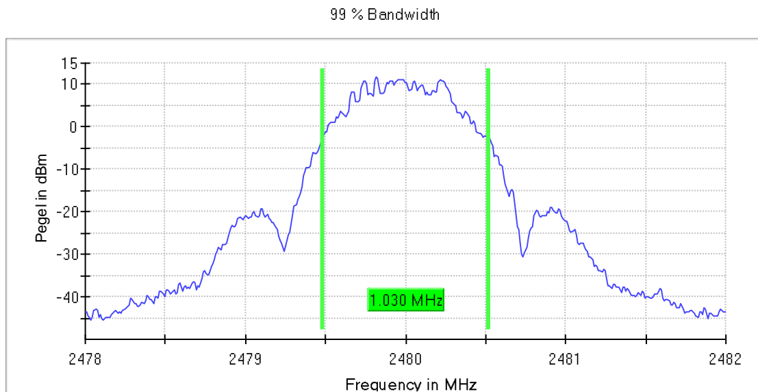
Transmission on 2480 MHz; - 40°C, 24 V DC
