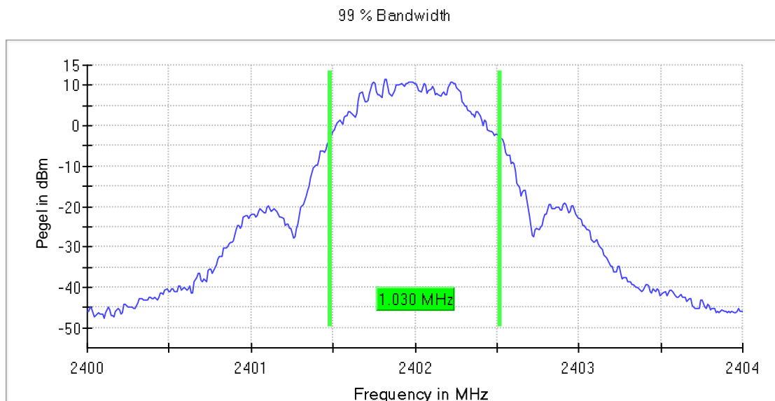
Transmission on 2402 MHz; - 40°C, 24 V DC
