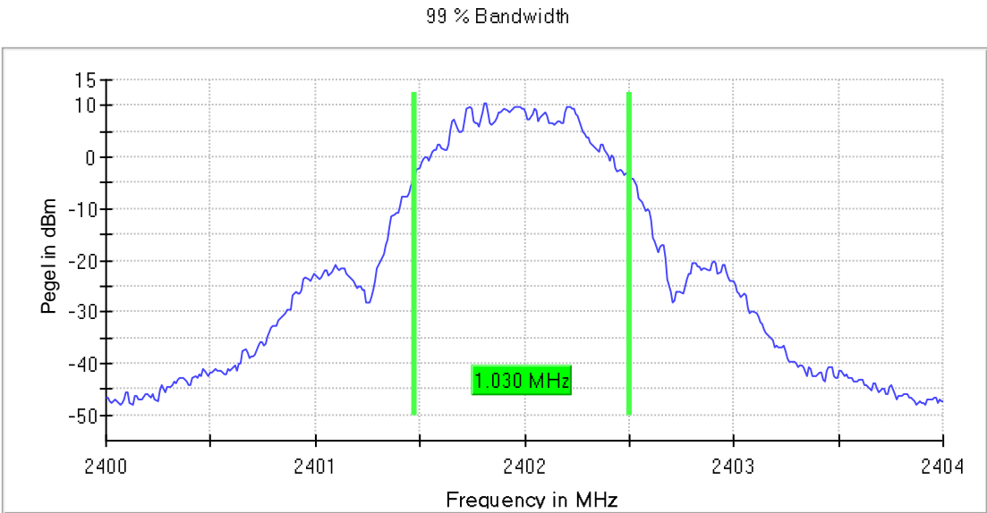
Transmission on 2402 MHz; + 85°C, 24 V DC
