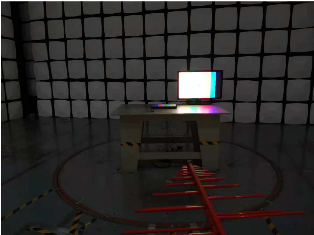
Radiated Emission Below 1GHz View- TAV-15
