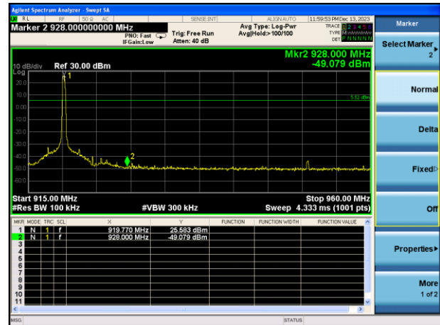
LORA: Band Edge-High Channel (Hopping Mode)
