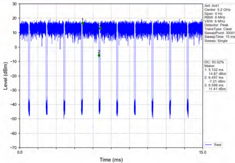
802.11ac(VHT20)_HCH_5240MHz_Ant1_NTNV
