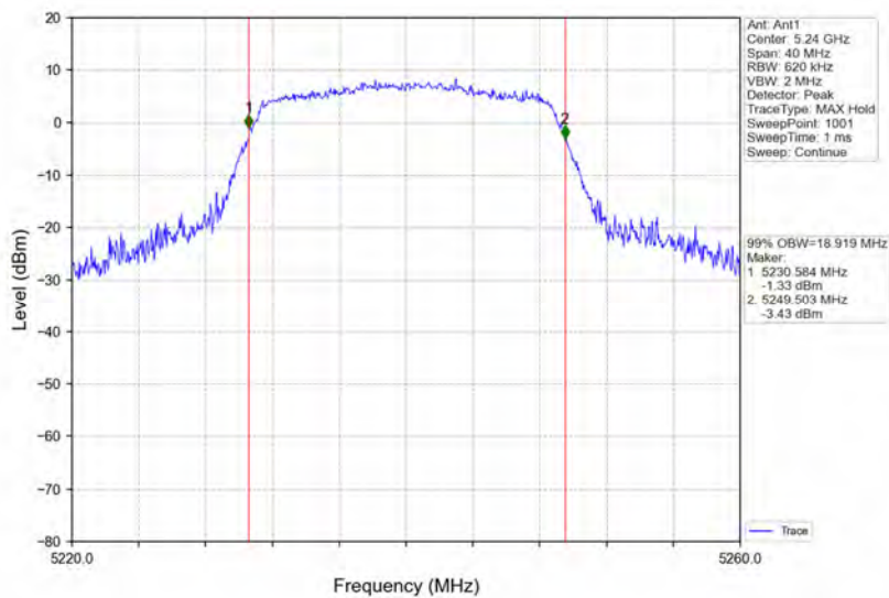
802.11ac(VHT20)_HCH_5240MHz_Ant1_NTNV
