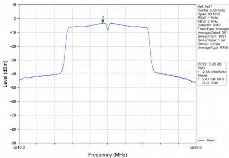
802.11ac(VHT40)_MCH_5550MHz_Ant1_NTNV
