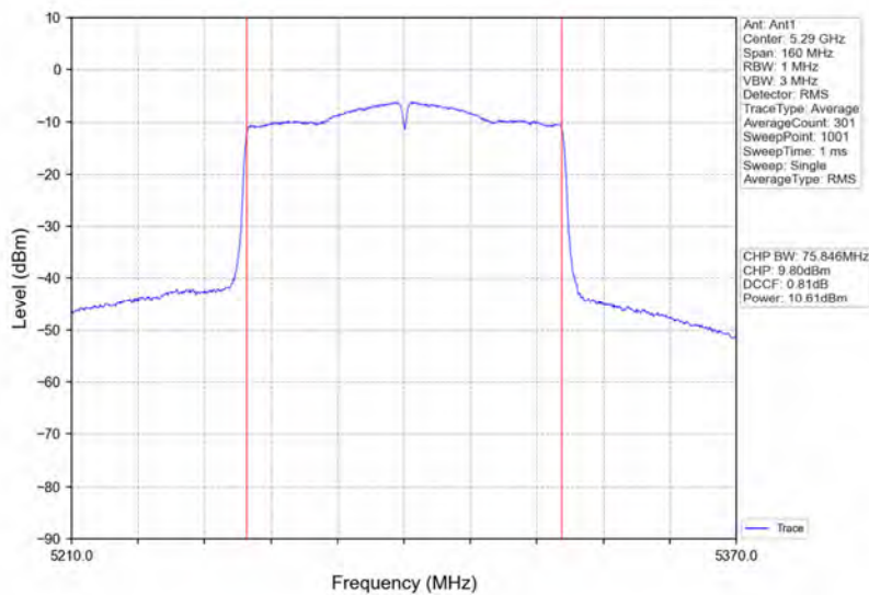
802.11ac(VHT80)_MCH_5290MHz_Ant1_NTNV
