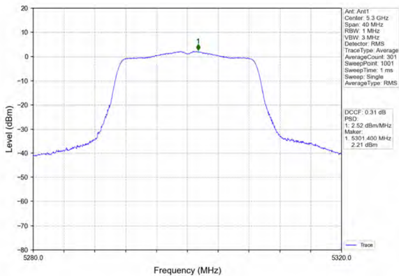
802.11ac(VHT20)_MCH_5300MHz_Ant1_NTNV
