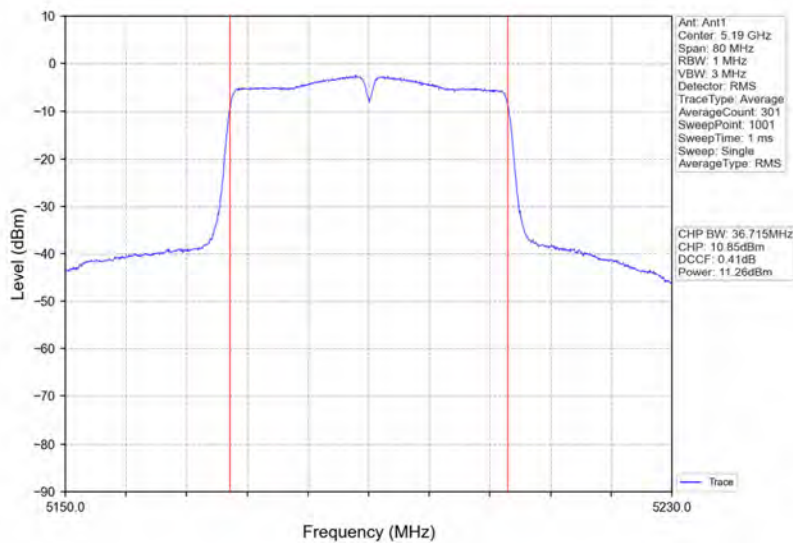
802.11ac(VHT40)_LCH_5190MHz_Ant1_NTNV
