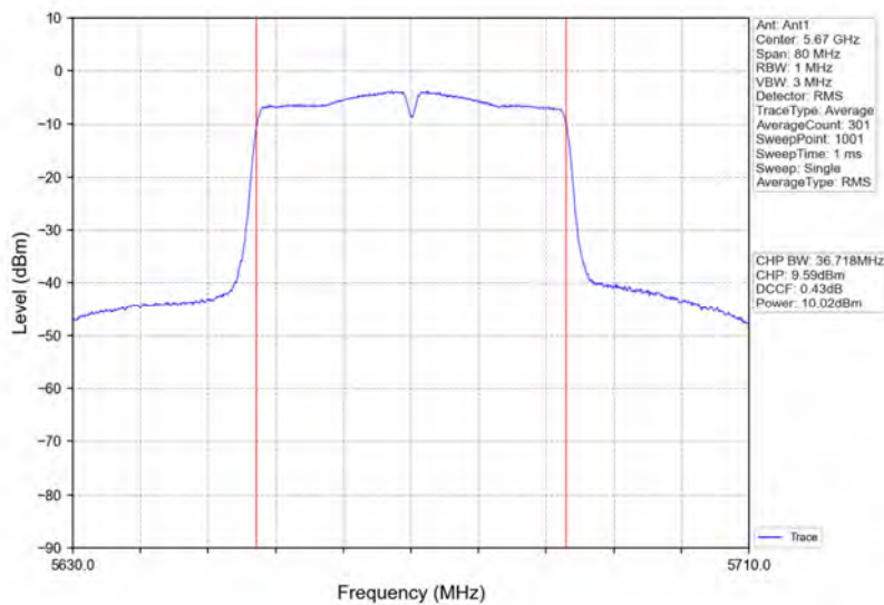
802.11ac(VHT40)_HCH_5670MHz_Ant1_NTNV
