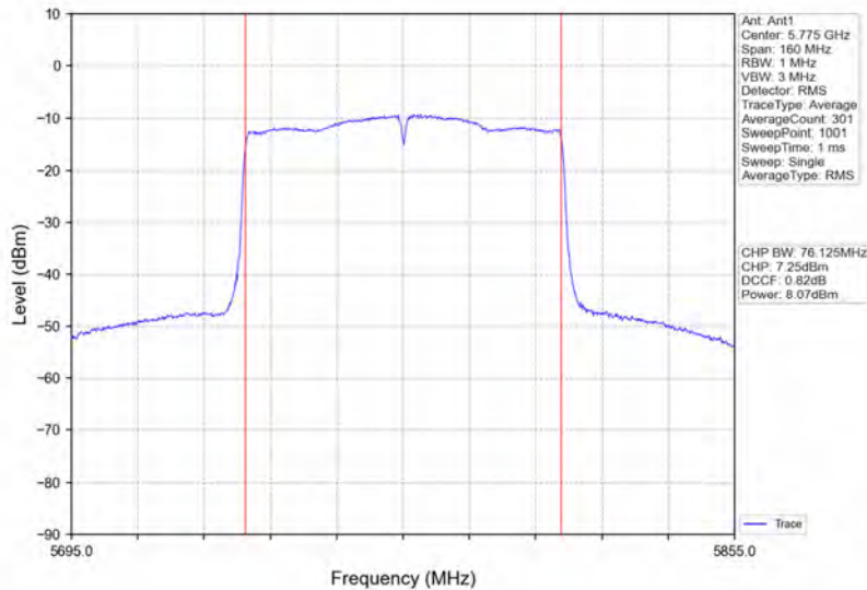
802.11ac(VHT80)_MCH_5775MHz_Ant1_NTNV
