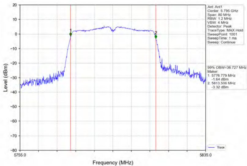
802.11ac(VHT40)_HCH_5795MHz_Ant1_NTNV
