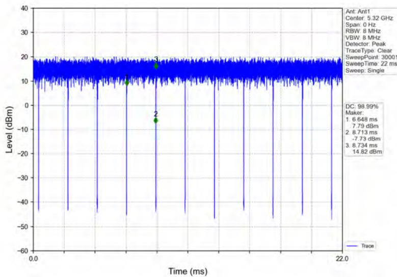
802.11a_HCH_5320MHz_Ant1_NTNV
