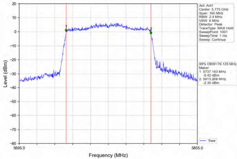
802.11ac(VHT80)_MCH_5775MHz_Ant1_NTNV
