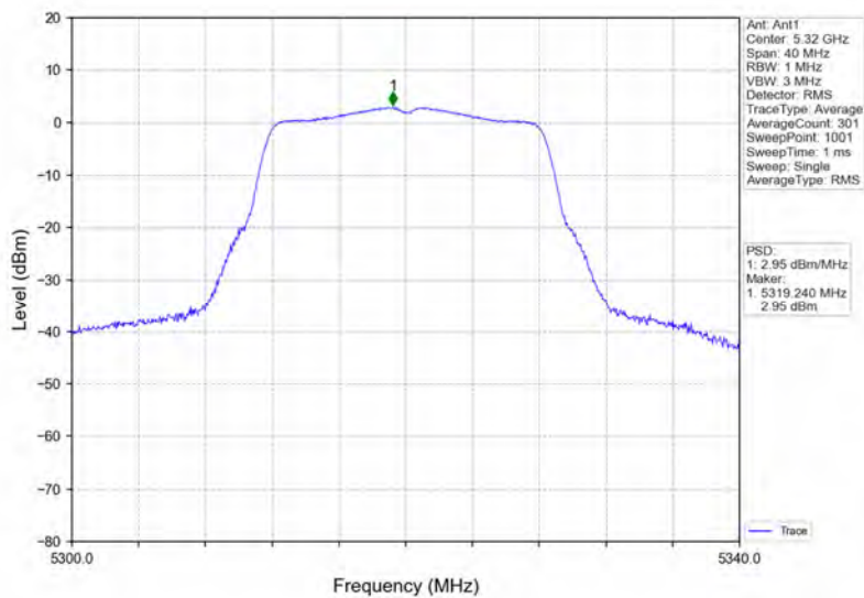
802.11a_HCH_5320MHz_Ant1_NTNV
