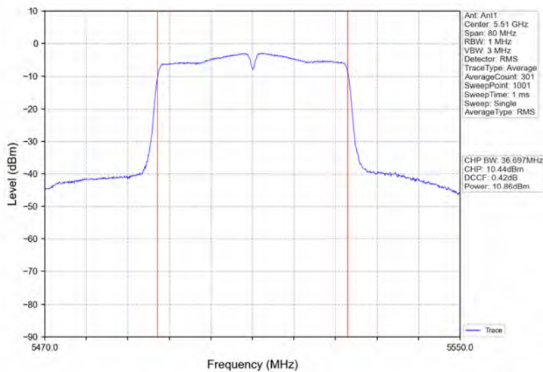
802.11ac(VHT40)_LCH_5510MHz_Ant1_NTNV
