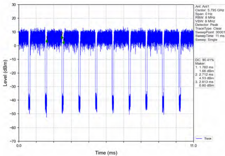
802.11ac(VHT40)_HCH_5795MHz_Ant1_NTNV
