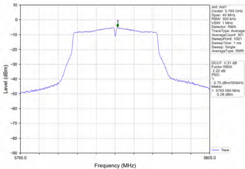
802.11ac(VHT20)_MCH_5785MHz_Ant1_NTNV
