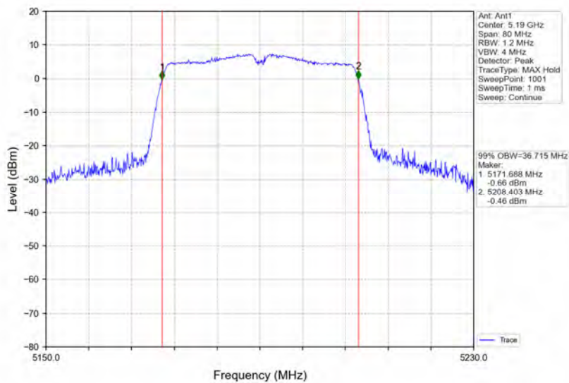
802.11ac(VHT40)_LCH_5190MHz_Ant1_NTNV
