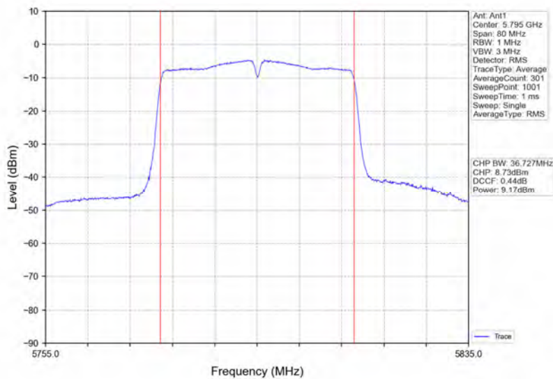
802.11ac(VHT40)_HCH_5795MHz_Ant1_NTNV
