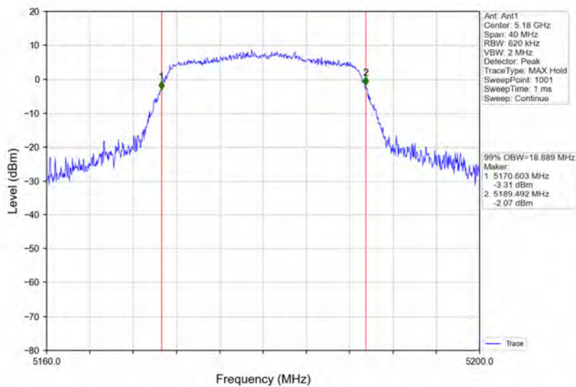
802.11ac(VHT20)_LCH_5180MHz_Ant1_NTNV
