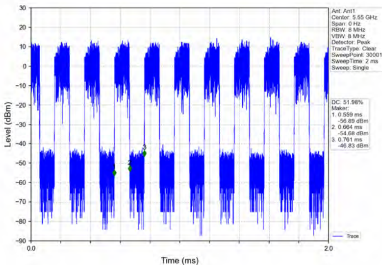
802.11n(HT40)_MCH_5550MHz_Ant1_NTNV
