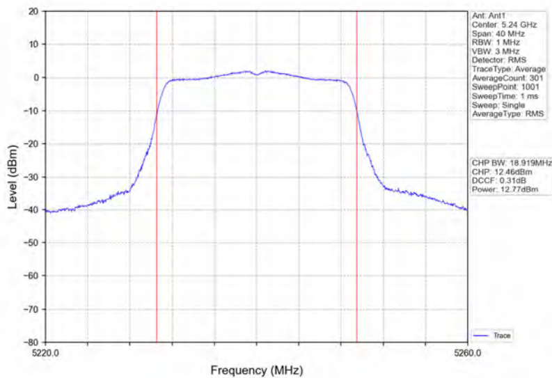
802.11ac(VHT20)_HCH_5240MHz_Ant1_NTNV
