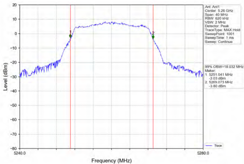
802.11a_LCH_5260MHz_Ant1_NTNV
