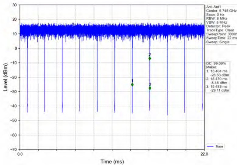
802.11a_LCH_5745MHz_Ant1_NTNV
