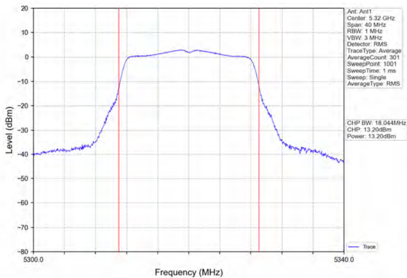
802.11a_HCH_5320MHz_Ant1_NTNV
