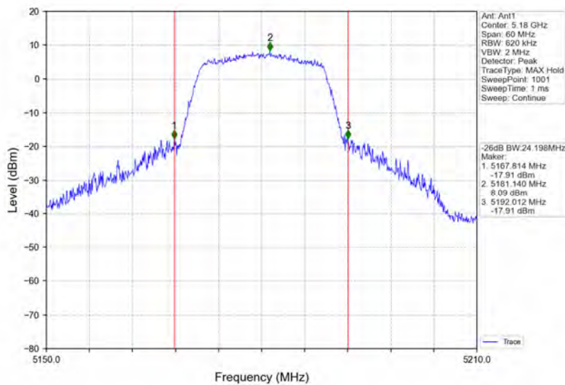
802.11ac(VHT20)_LCH_5180MHz_Ant1_NTNV
