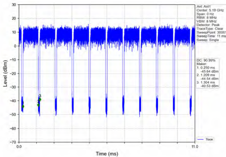
802.11ac(VHT40)_LCH_5190MHz_Ant1_NTNV
