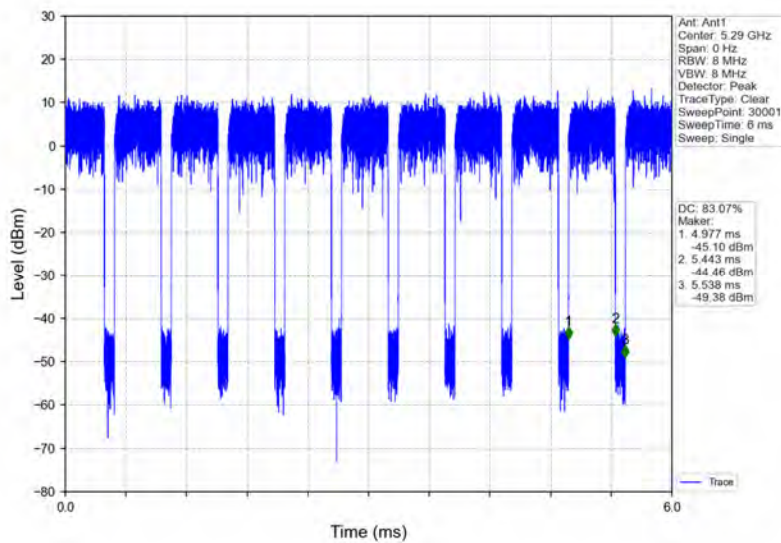
802.11ac(VHT80)_MCH_5290MHz_Ant1_NTNV
