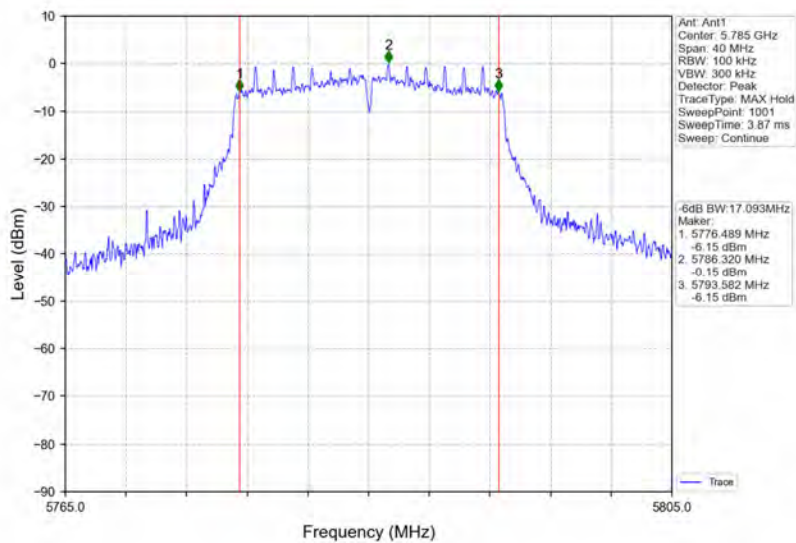
802.11ac(VHT20)_MCH_5785MHz_Ant1_NTNV
