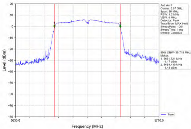
802.11ac(VHT40)_HCH_5670MHz_Ant1_NTNV
