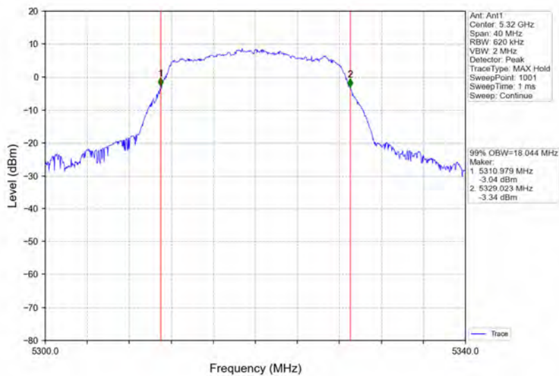
802.11a_HCH_5320MHz_Ant1_NTNV
