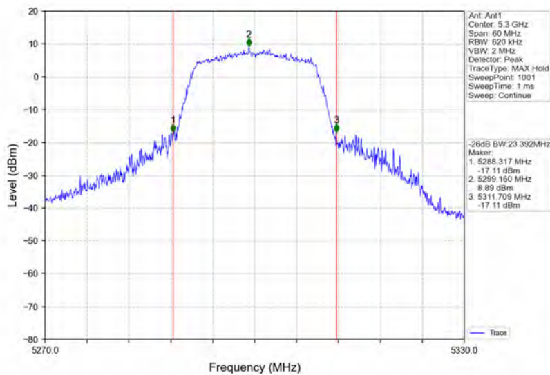
802.11n(HT20)_MCH_5300MHz_Ant1_NTNV
