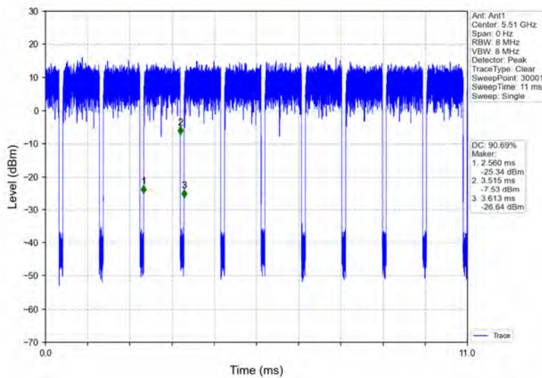
802.11ac(VHT40)_LCH_5510MHz_Ant1_NTNV
