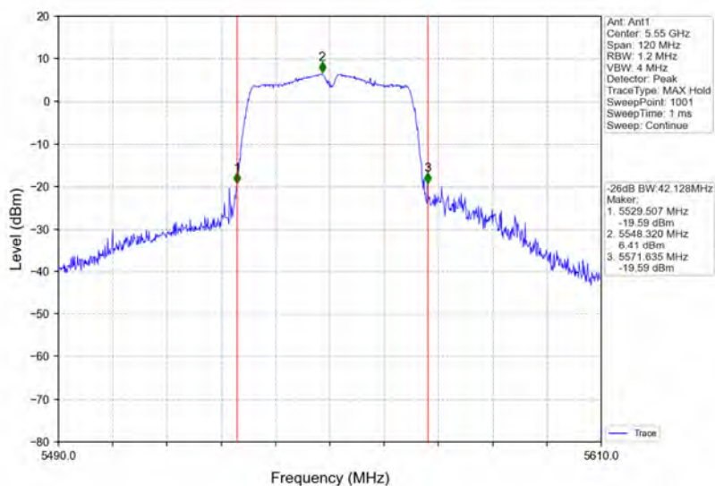
802.11ac(VHT40)_MCH_5550MHz_Ant1_NTNV
