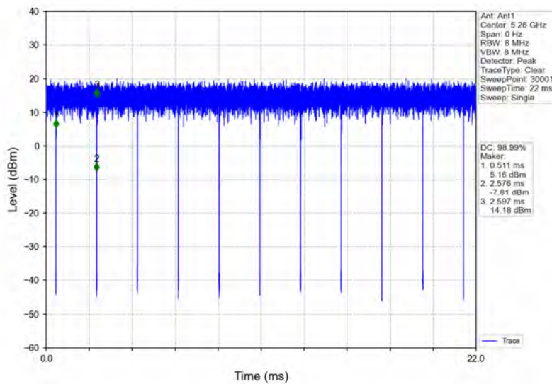
802.11a_LCH_5260MHz_Ant1_NTNV
