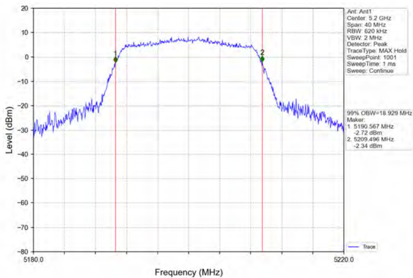
802.11n(HT20)_MCH_5200MHz_Ant1_NTNV
