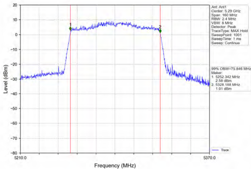
802.11ac(VHT80)_MCH_5290MHz_Ant1_NTNV
