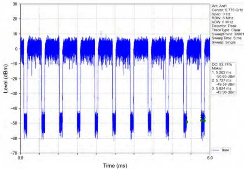
802.11ac(VHT80)_MCH_5775MHz_Ant1_NTNV
