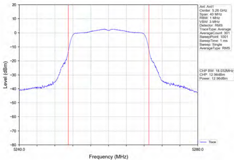
802.11a_LCH_5260MHz_Ant1_NTNV
