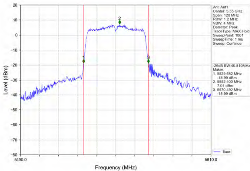
802.11n(HT40)_MCH_5550MHz_Ant1_NTNV
