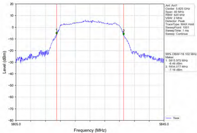
802.11a_HCH_5825MHz_Ant1_NTNV
