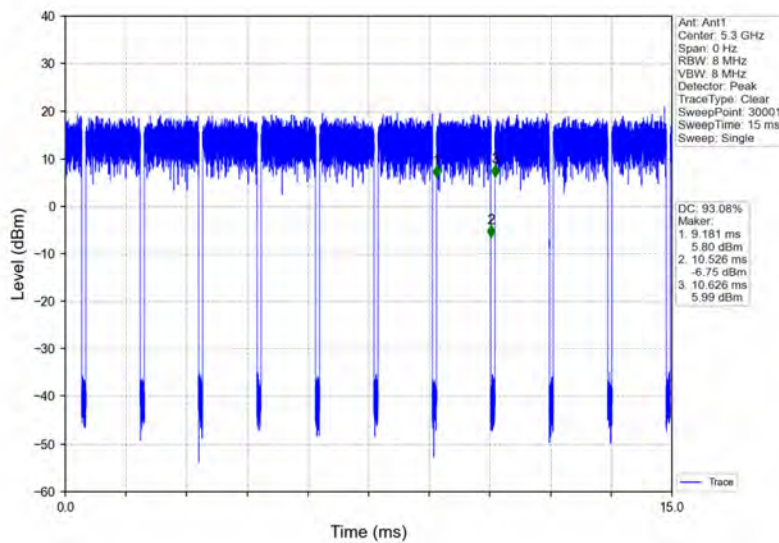
802.11ac(VHT20)_MCH_5300MHz_Ant1_NTNV
