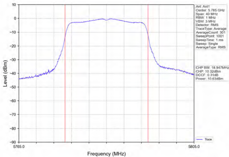
802.11ac(VHT20)_MCH_5785MHz_Ant1_NTNV
