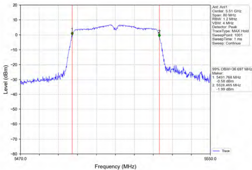
802.11ac(VHT40)_LCH_5510MHz_Ant1_NTNV
