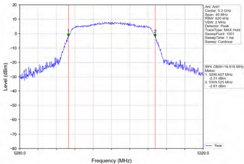
802.11ac(VHT20)_MCH_5300MHz_Ant1_NTNV
