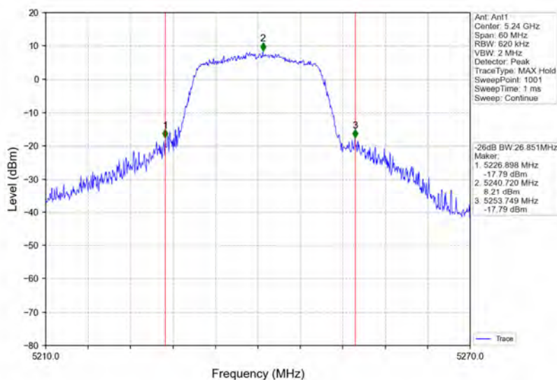
802.11ac(VHT20)_HCH_5240MHz_Ant1_NTNV
