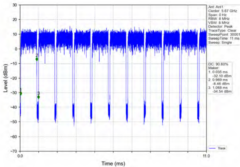
802.11ac(VHT40)_HCH_5670MHz_Ant1_NTNV
