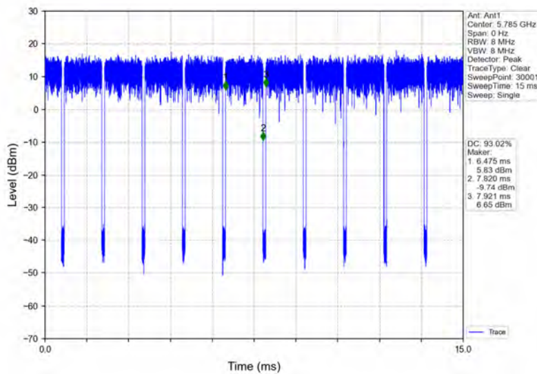
802.11ac(VHT20)_MCH_5785MHz_Ant1_NTNV
