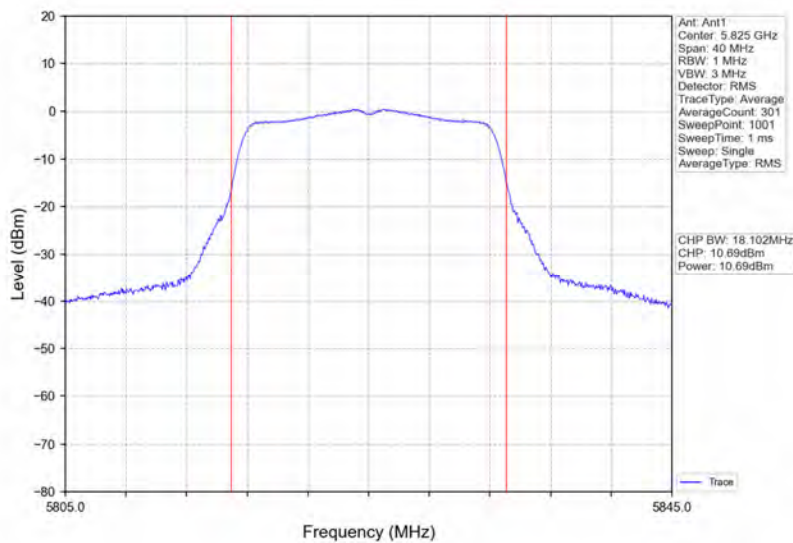
802.11a_HCH_5825MHz_Ant1_NTNV
