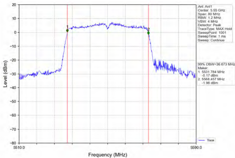
802.11n(HT40)_MCH_5550MHz_Ant1_NTNV
