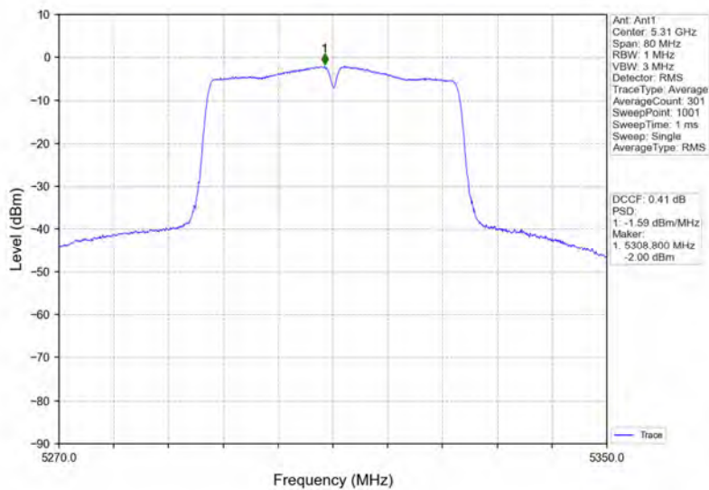
802.11ac(VHT40)_HCH_5310MHz_Ant1_NTNV
