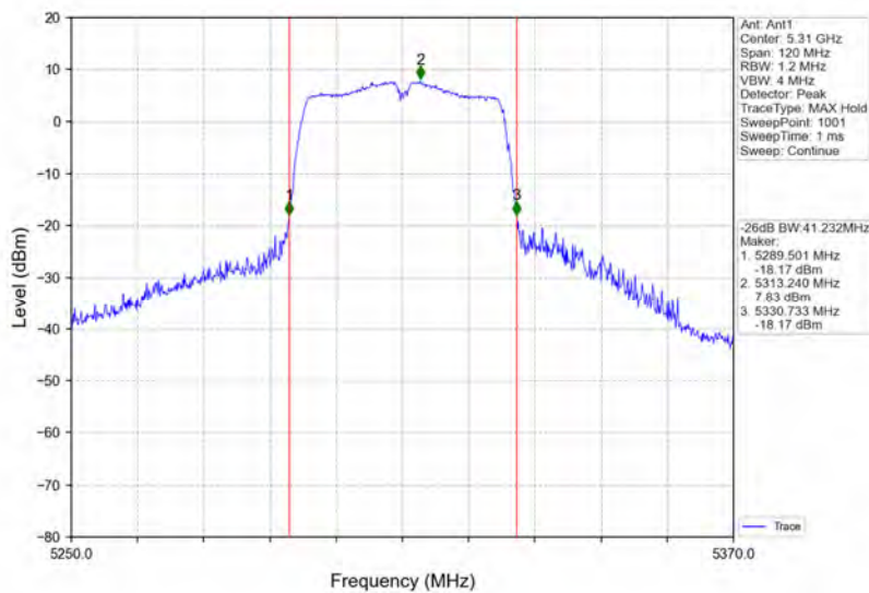
802.11ac(VHT40)_HCH_5310MHz_Ant1_NTNV
