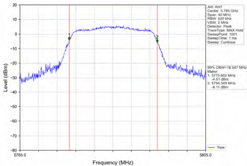
802.11ac(VHT20)_MCH_5785MHz_Ant1_NTNV
