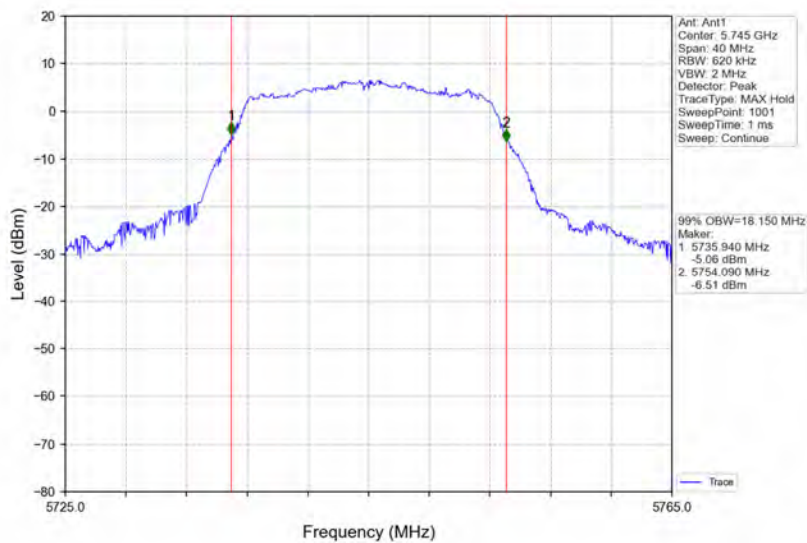
802.11a_LCH_5745MHz_Ant1_NTNV
