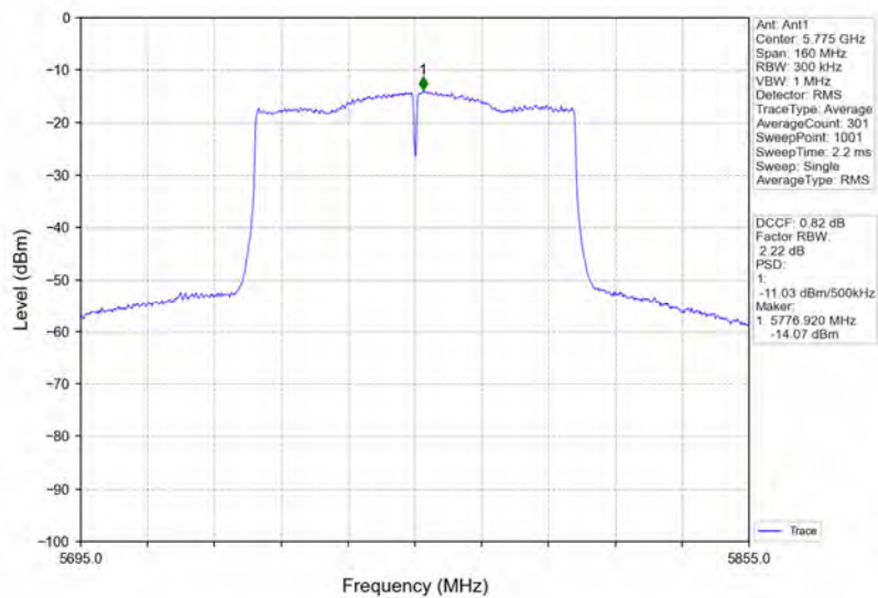
802.11ac(VHT80)_MCH_5775MHz_Ant1_NTNV
