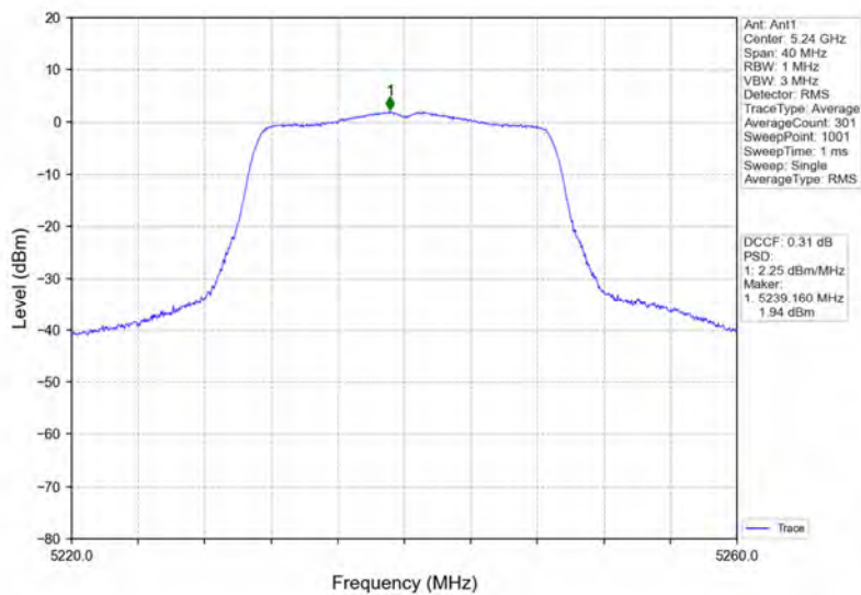
802.11ac(VHT20)_HCH_5240MHz_Ant1_NTNV
