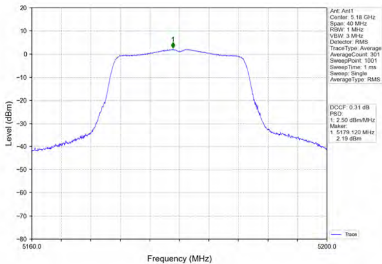
802.11ac(VHT20)_LCH_5180MHz_Ant1_NTNV
