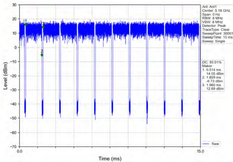
802.11ac(VHT20)_LCH_5180MHz_Ant1_NTNV
