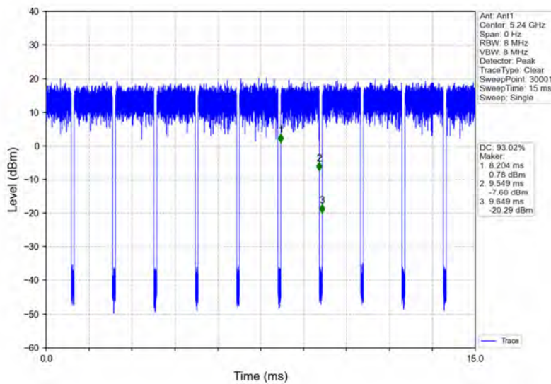
802.11ac(VHT20)_HCH_5240MHz_Ant1_NTNV
