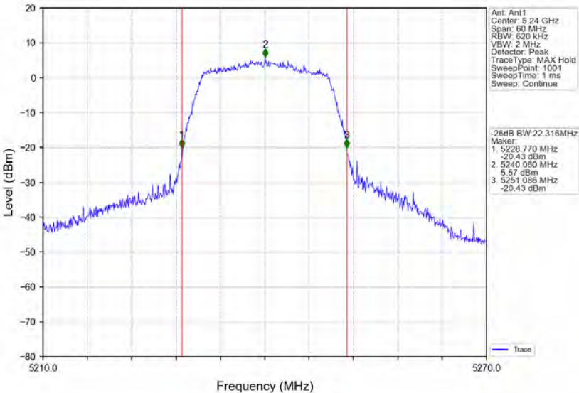
802.11ac(VHT20)_HCH_5240MHz_Ant1_NTNV
