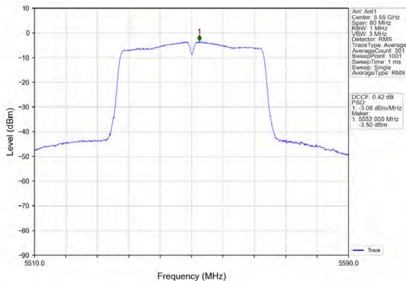
802.11ac(VHT40)_MCH_5550MHz_Ant1_NTNV
