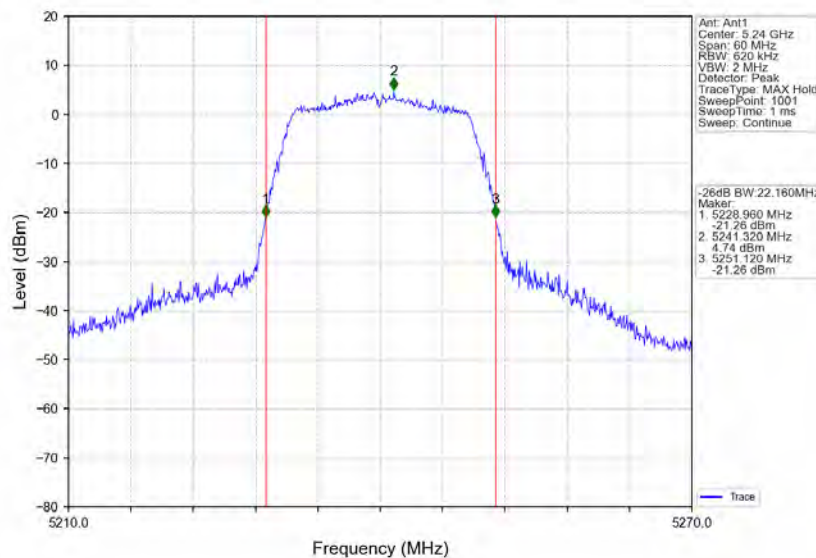
802.11n(HT20)_HCH_5240MHz_Ant1_NTNV
