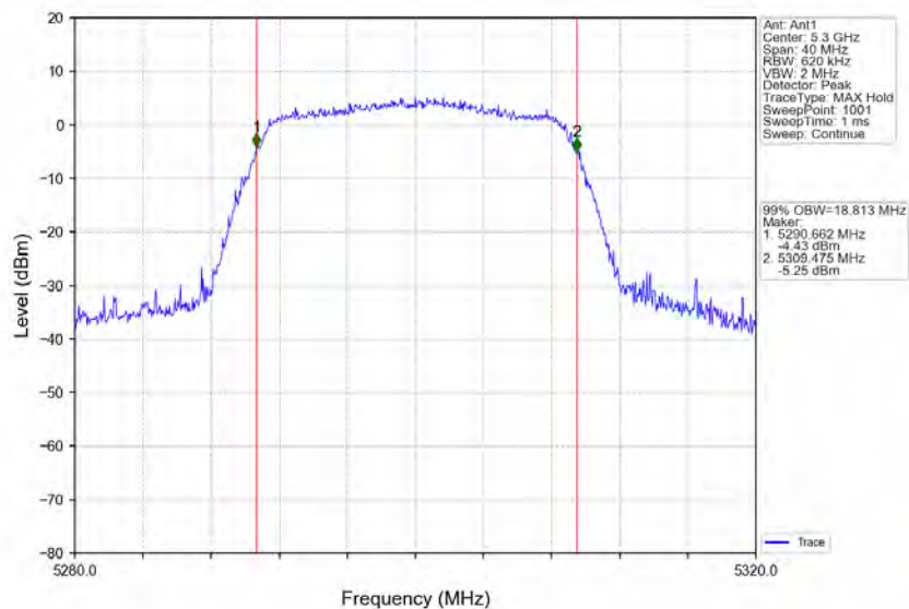
802.11ac(VHT20)_MCH_5300MHz_Ant1_NTNV
