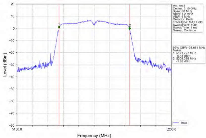
802.11ac(VHT40)_LCH_5190MHz_Ant1_NTNV
