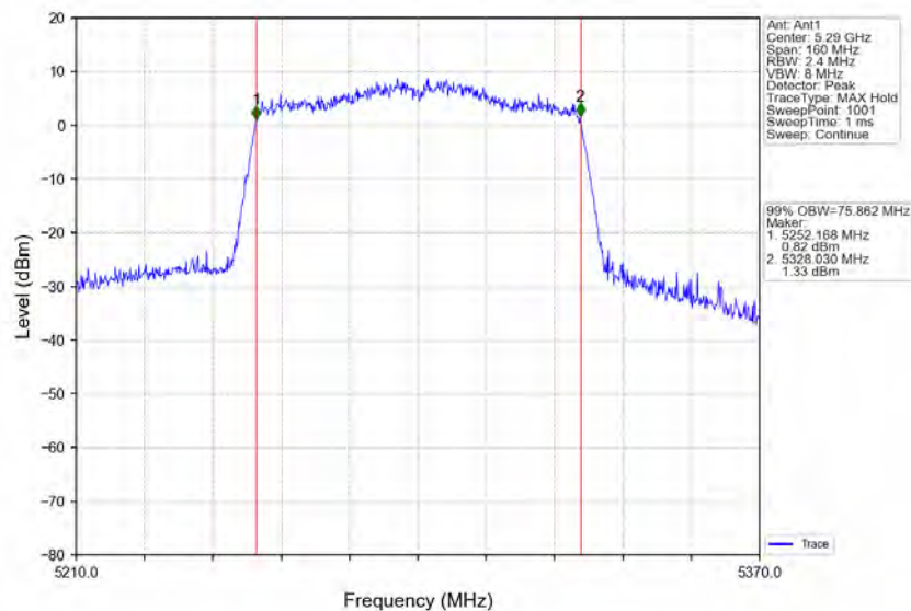
802.11ac(VHT80)_MCH_5290MHz_Ant1_NTNV
