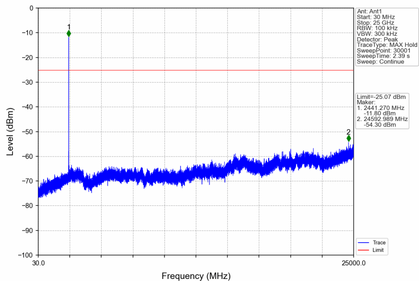
Pi/4DQPSK_2DH5_MCH_2441MHz_Ant1_NTNV
