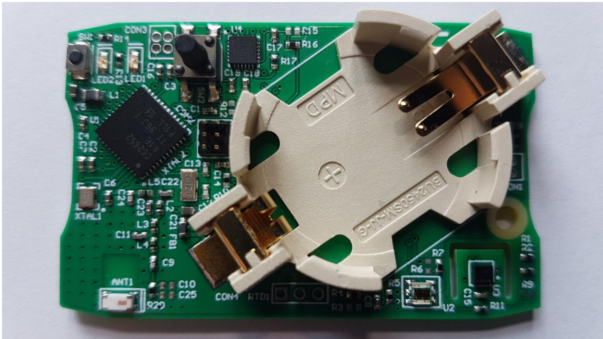
TP-100-TH Circuit Card Top
