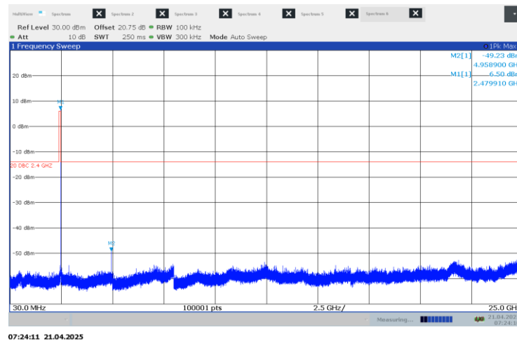
Figure 7.6-19: Conducted spurious emissions at high ch
