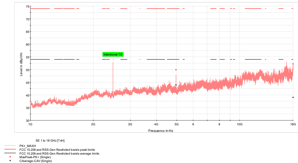
Figure 7.6-6: Radiated spurious emissions 1-18 GHz high channel
