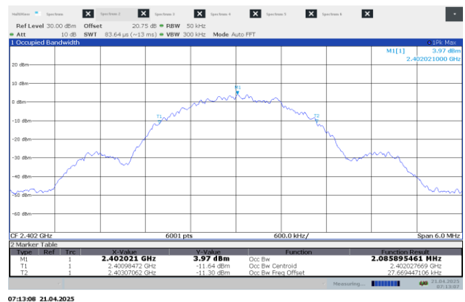
Figure 7.4-4: 99% occupied bandwidth on low ch
