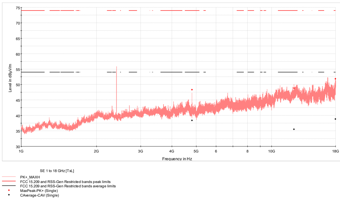
Figure 7.6-4: Radiated spurious emissions 1-18 GHz low channel
