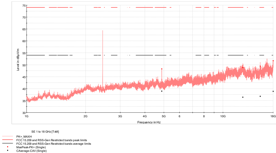
Figure 7.6-5: Radiated spurious emissions 1-18 GHz mid channel
