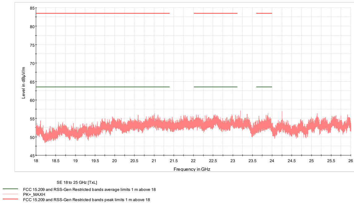
Figure 7.6-8: Radiated spurious emissions 18-26 GHz low channel
