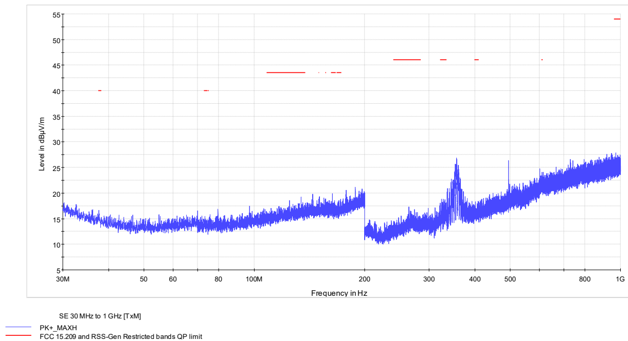
Figure 7.6-2: Radiated spurious emissions 30-1000 MHz mid channel
