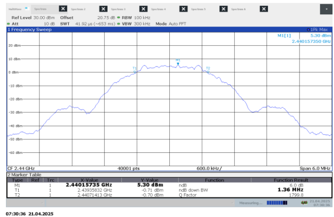
Figure 7.4-2: 6 dB bandwidth on mid ch
