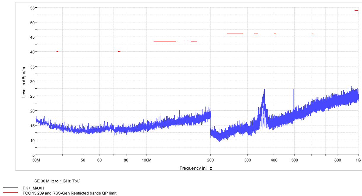
Figure 7.6-1: Radiated spurious emissions 30-1000 MHz low channel
