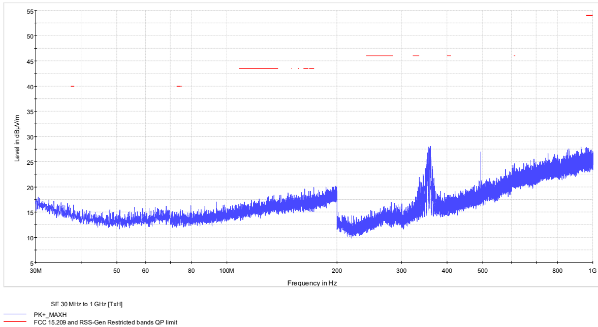
Figure 7.6-3: Radiated spurious emissions 30-1000 MHz high channel
