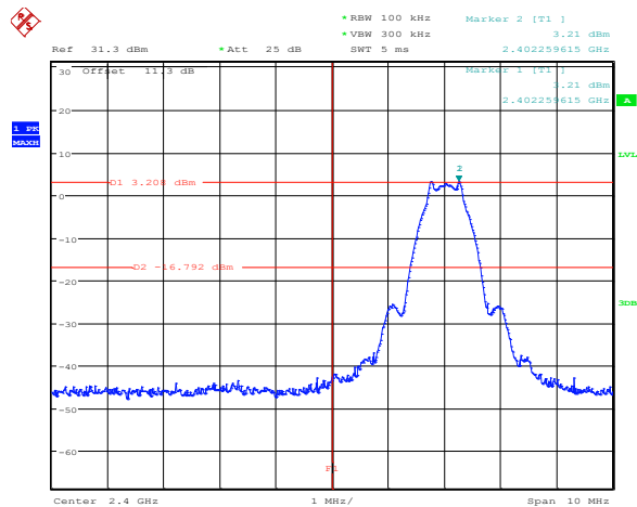
Figure 8.7-4: Conducted spurious (out-of-band) emissions Lower band, low channel)
