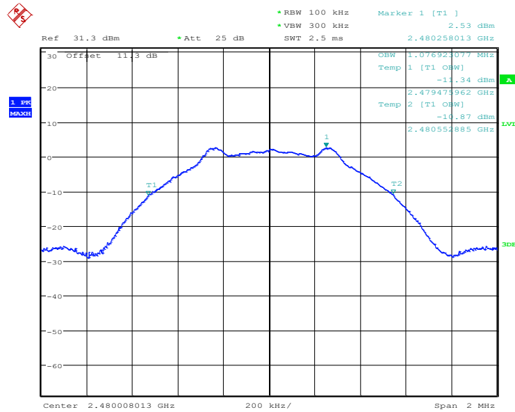
Figure 8.5-6: 99% dB bandwidth on high channel
