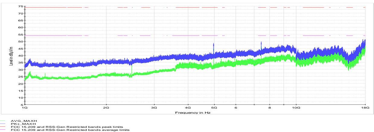
Figure 8.7-13: Radiated spurious (out-of-band) emissions, Above 1 GHz, high channel
