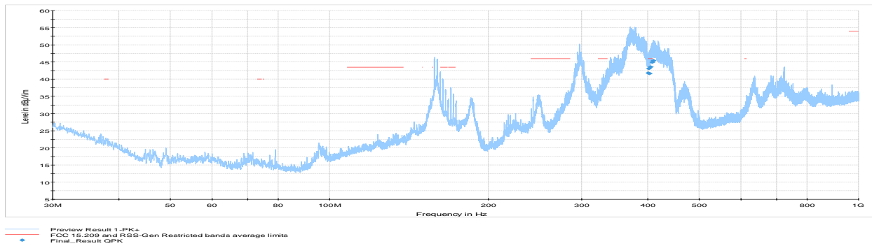
Figure 8.7-9: Radiated spurious (out-of-band) emissions, below 1 GHz, Mid channel
