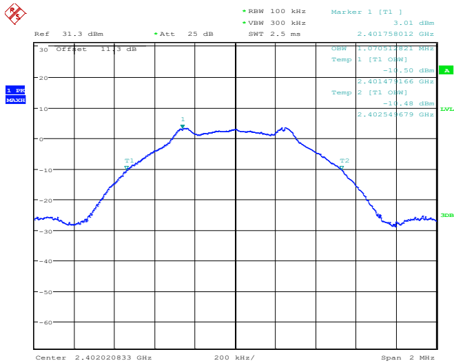
Figure 8.5-4: 99% dB bandwidth on low channel
