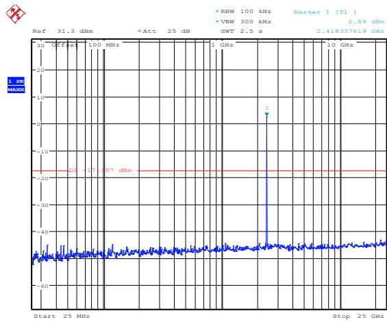
Figure 8.7-1: Conducted spurious (out-of-band) emissions, low channel
