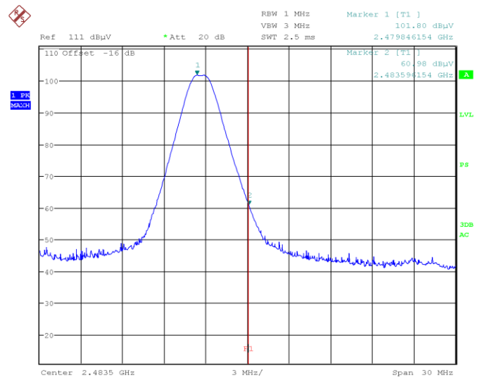
Figure 8.7-7: Radiated spurious (out-of-band) emissions upper band, high channel
