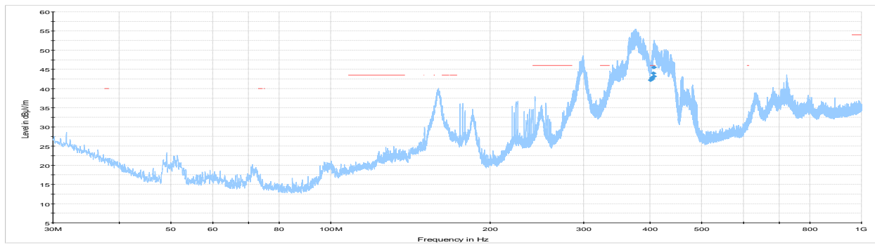
Figure 8.7-10: Radiated spurious (out-of-band) emissions, below 1 GHz, high channel
