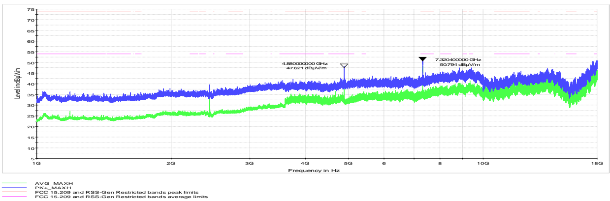
Figure 8.7-12: Radiated spurious (out-of-band) emissions, Above 1 GHz, Mid channel
