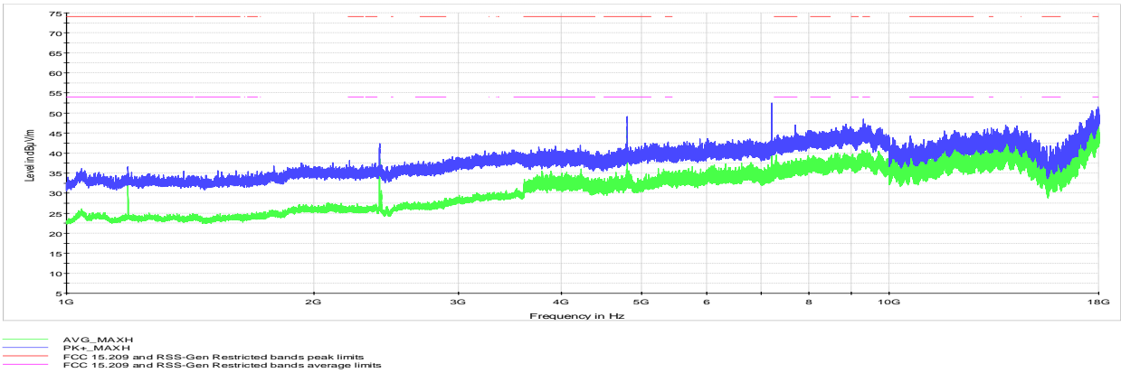
Figure 8.7-11: Radiated spurious (out-of-band) emissions, Above 1 GHz, Low channel
