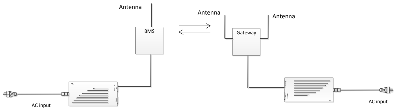
Figure 5.5-1: Test setup block diagram
