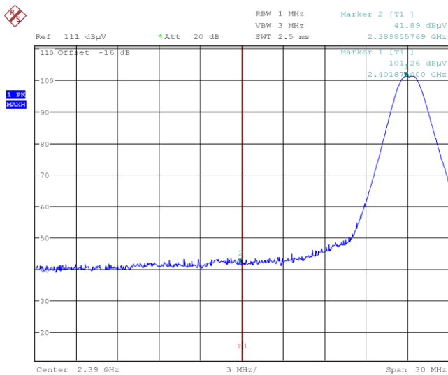
Figure 8.7-6: Radiated spurious (out-of-band) emissions Lower band, low channel)
