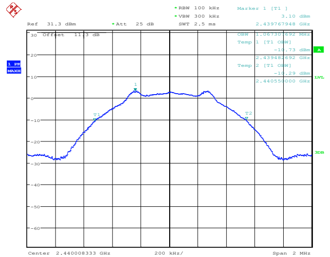
Figure 8.5-5: 99% dB bandwidth on mid channel
