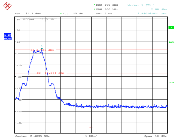
Figure 8.7-5: Conducted spurious (out-of-band) emissions upper band, high channel
