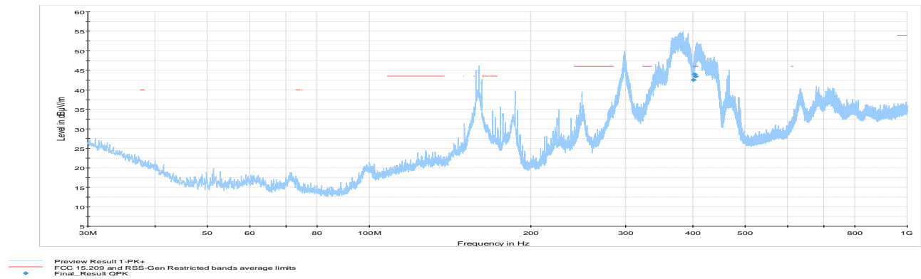
Figure 8.7-8: Radiated spurious (out-of-band) emissions, below 1 GHz, Low channel
