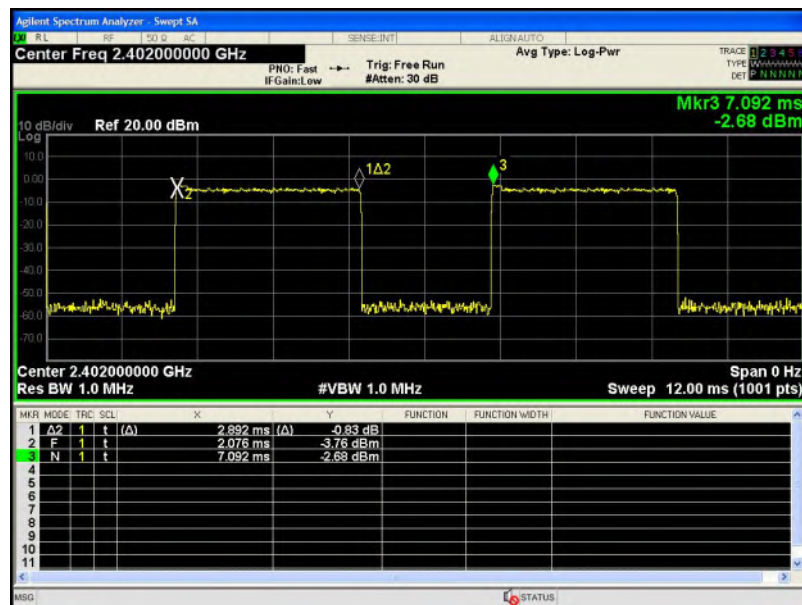
Test Mode: EDR---3DH5
