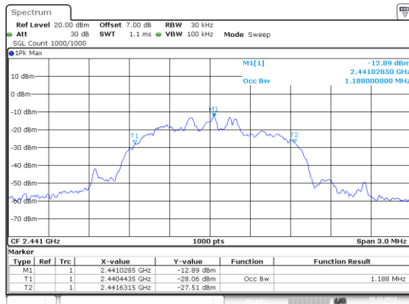
2DH1_Middle 1.188MHz
