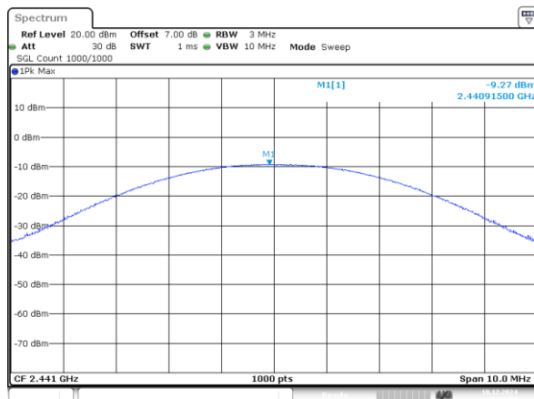
2DH1_Middle -9.27dBm
