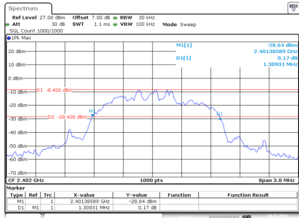
2DH1_Low 1.309MHz
