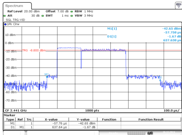
2DH1_Hopping 0.638ms
