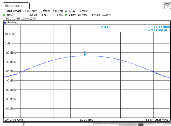
2DH1_High -13.42dBm
