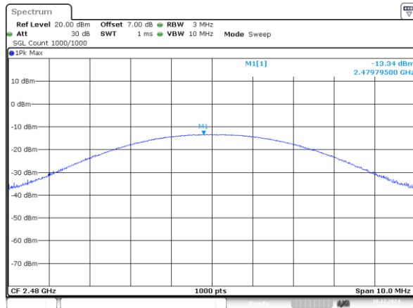
3DH1_High -13.34dBm
