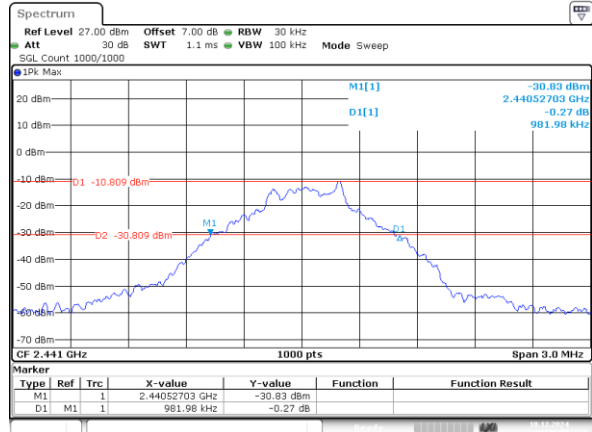
DH1_Middle 0.982MHz
