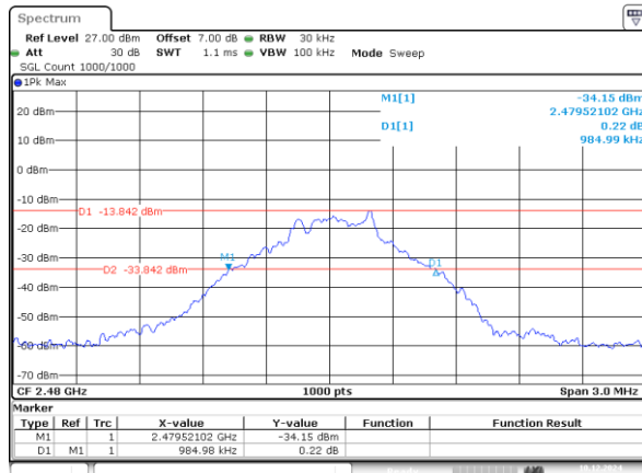
DH1_High 0.985MHz
