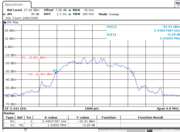
2DH1_Middle 1.318MHz
