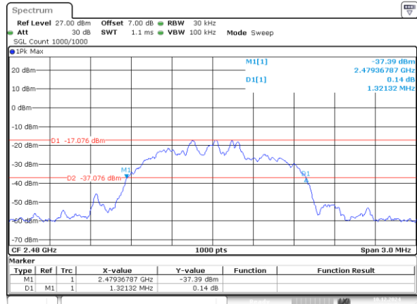
2DH1_High 1.321MHz
