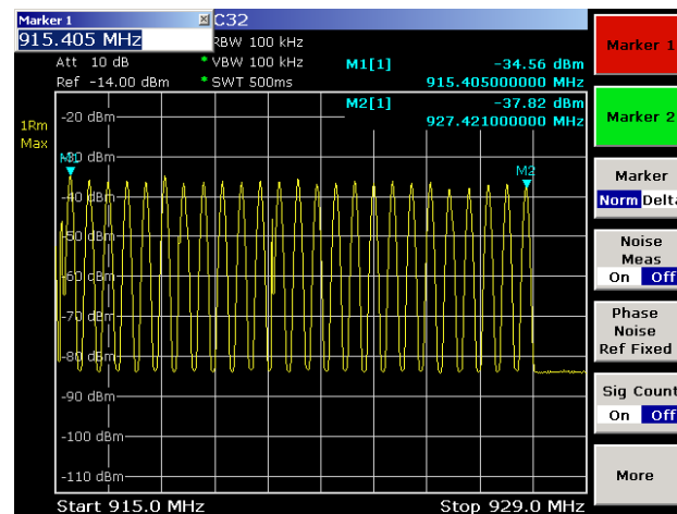
Plot # 13. Hopping channels.
