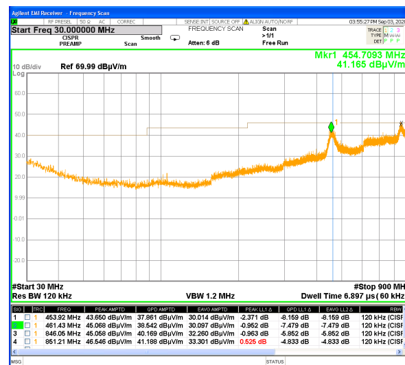
Plot # 59. Investigation result in 30 - 900 MHz frequency range.
