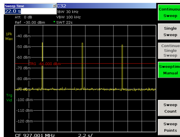
Plot # 15. Average time of occupancy
