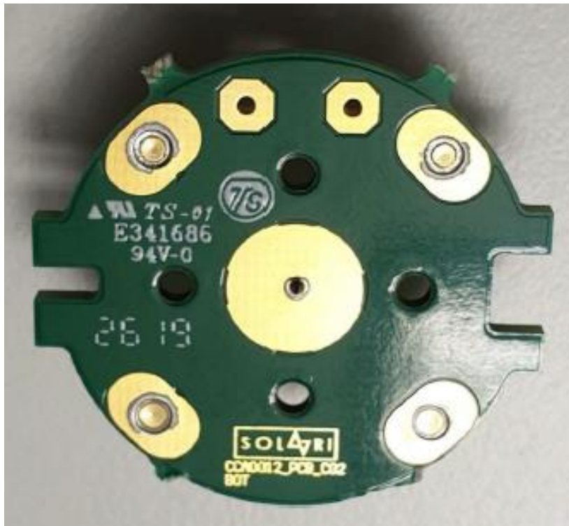
CCA0012_C02_TOP (Speaker-Board)
