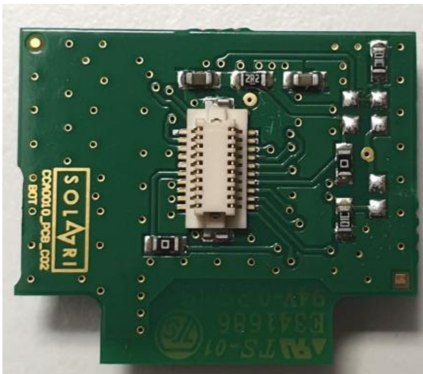
CCA0010_C02_BACK (BT-Board)
