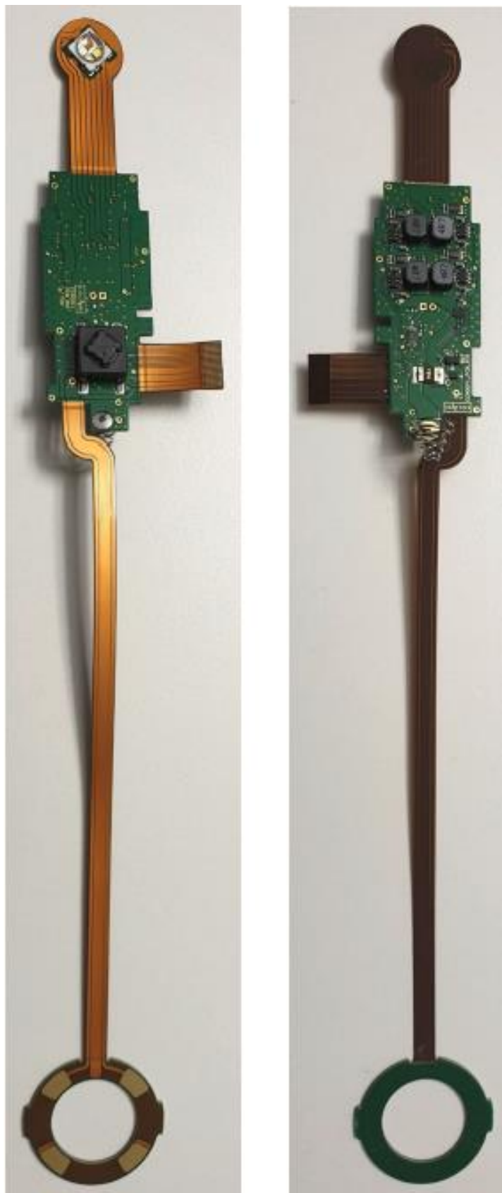
CCA0011_B02_TOP & BACK (LED-Board)
