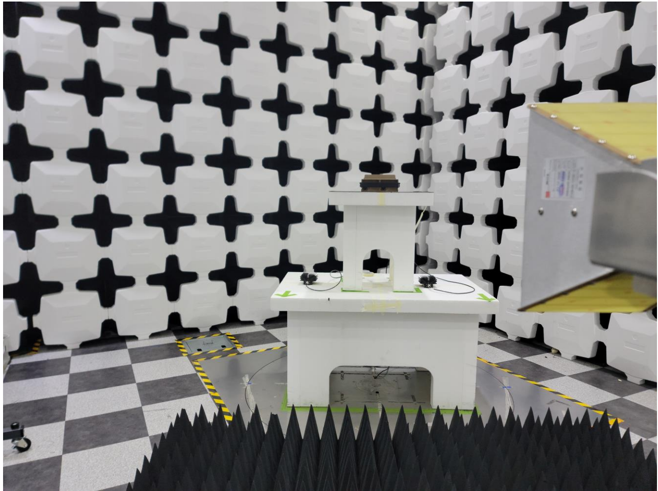
Above 1GHz Test Instrument & Measurement Setup
