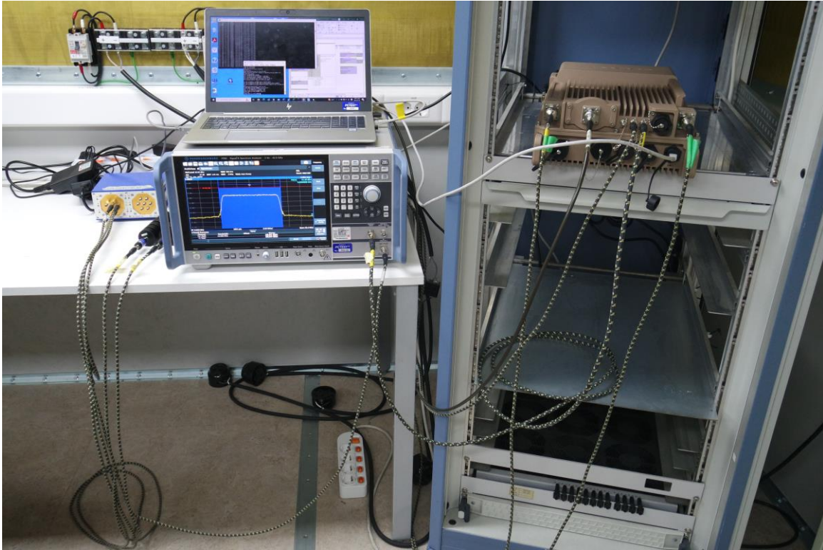
Conducted Test Instrument & Measurement Setup
