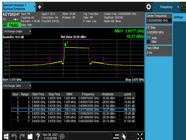
Plot 8-40. Channel Edge Emission Plot (LTE_B48_20M_16QAM – Mid Channel, Port 0)
