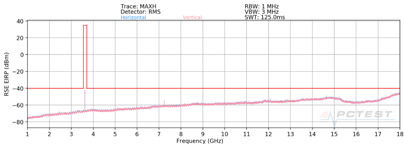
Plot 8-57. Radiated spurious emission Plot_1 GHz to 18 GHz (LTE_B48_20M_QPSK - Mid Channel)
