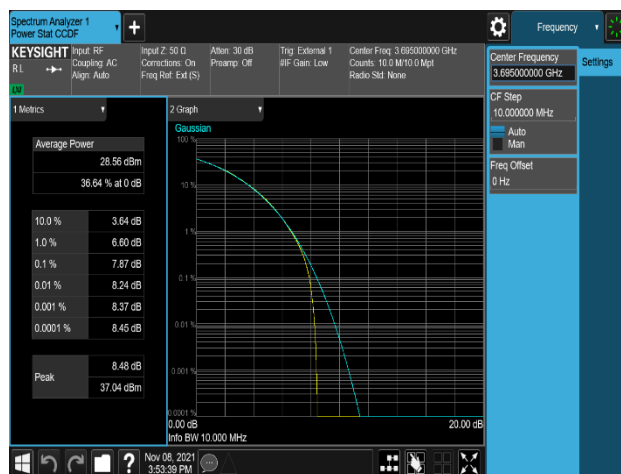
Plot 8-34. Peak To Average Power Ratio Plot (LTE_B48_10M_QPSK - High Channel, Port 1)
