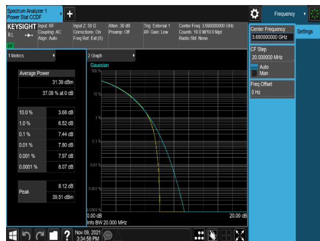
Plot 8-35. Peak To Average Power Ratio Plot (LTE_B48_20M_QPSK - High Channel, Port 1)
