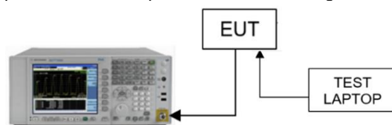
Figure 8-1. Test Instrument & Measurement Setup
