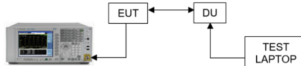
Figure 10-1. Test Instrument & Measurement Setup
