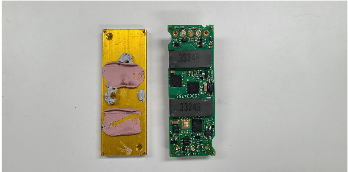
PSU_in DC-DC Converter top_Without shields
