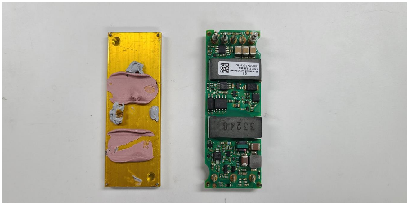
PSU-S_in DC-DC Converter Bottom_Without shields
