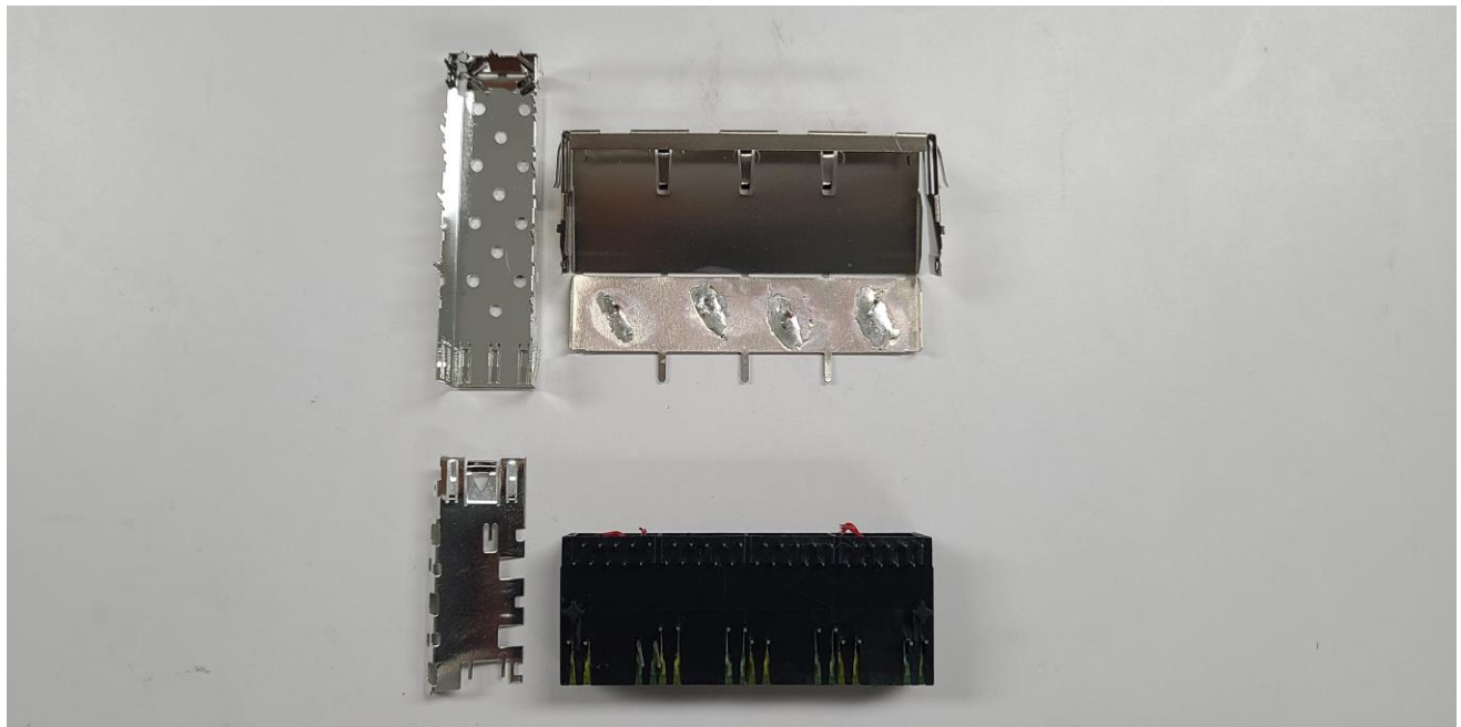
MDC in SFP cage & RJ 45 connector_bottom_Without shields
