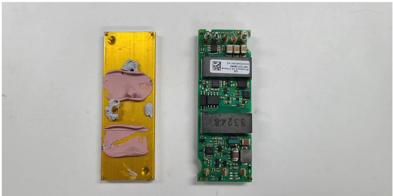
PSU_in DC-DC Converter Bottom_Without shields
