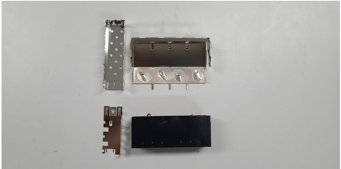
MDC in SFP cage & RJ 45 connector_top_Without shields
