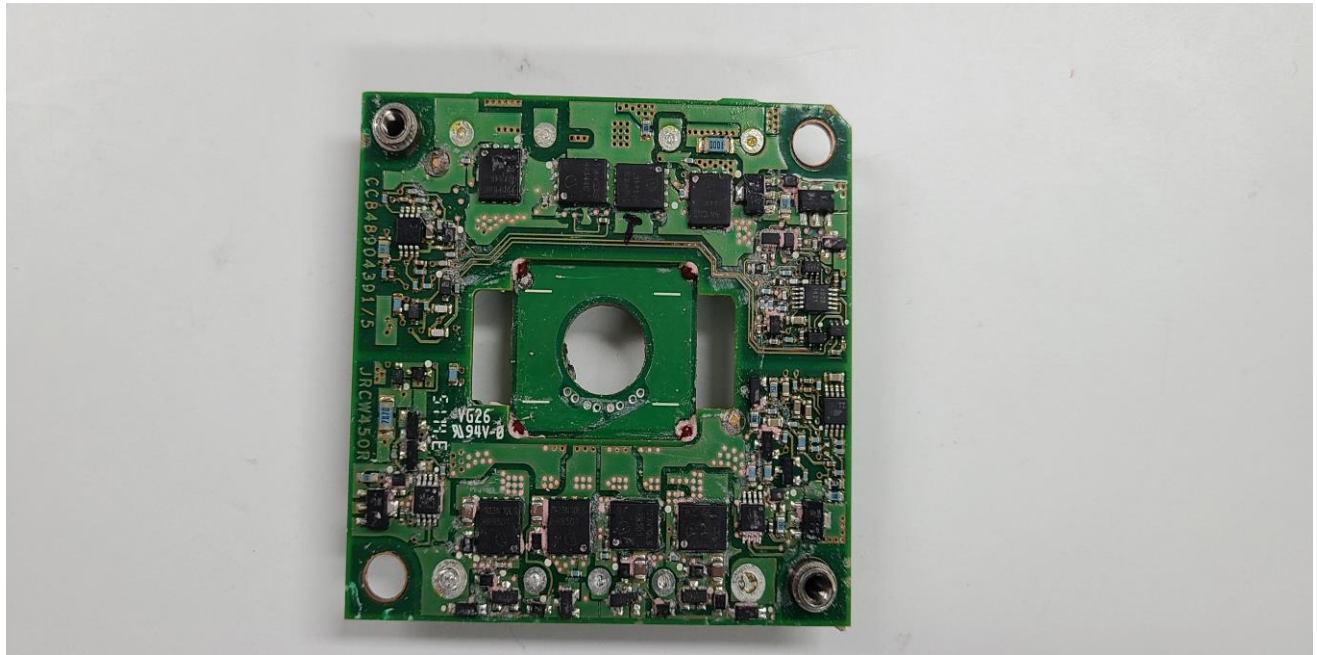
PSU_in DC-DC Converter top_Without shields
