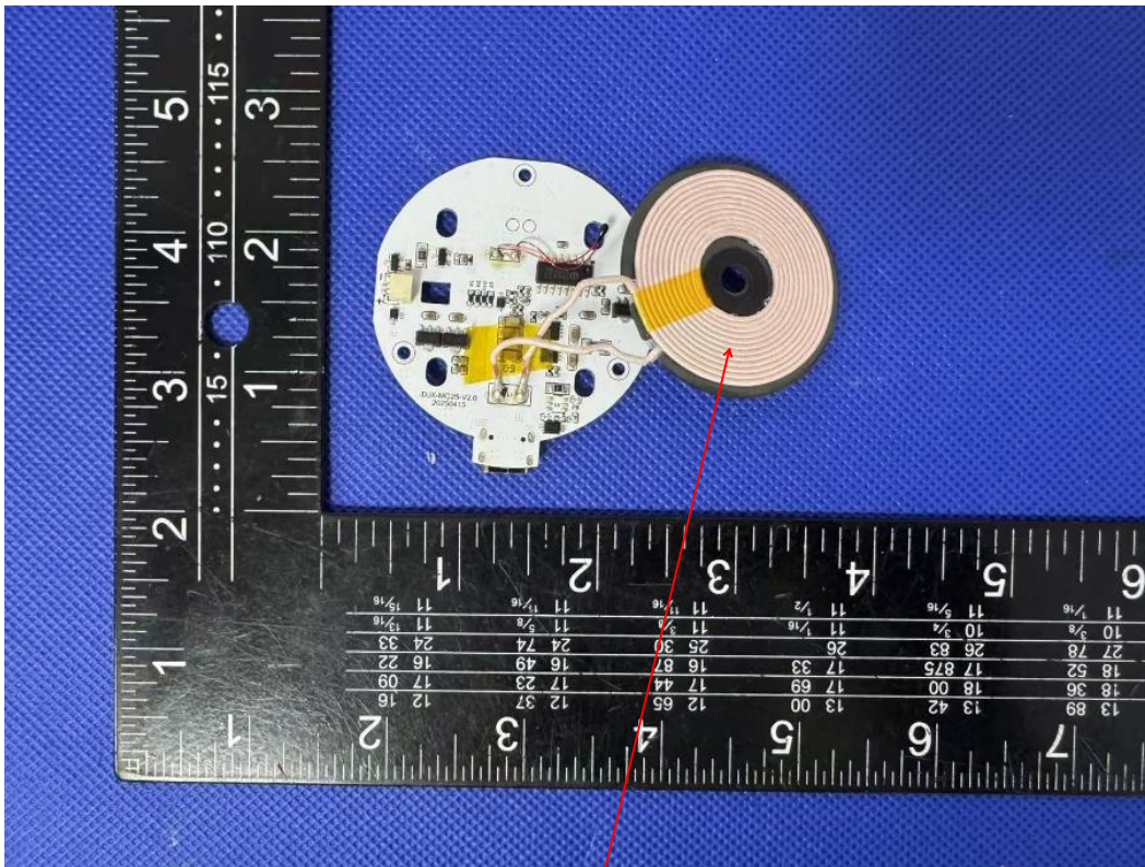
Loop Antenna
