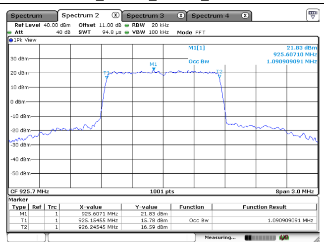
Cat-M1_1.4MHz_16QAM_925.7 MHz
