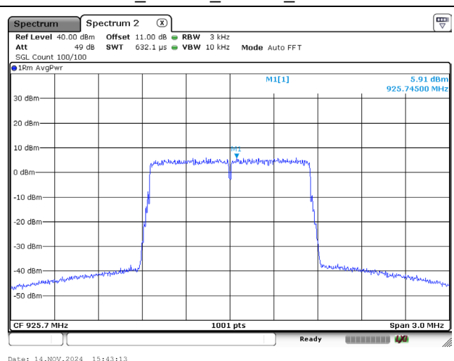
Cat-M1_1.4MHz_16QAM_925.7 MHz
