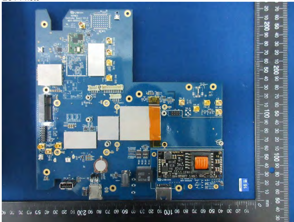
(24) EUT Photo (SD Card: DU3A-016GT)
