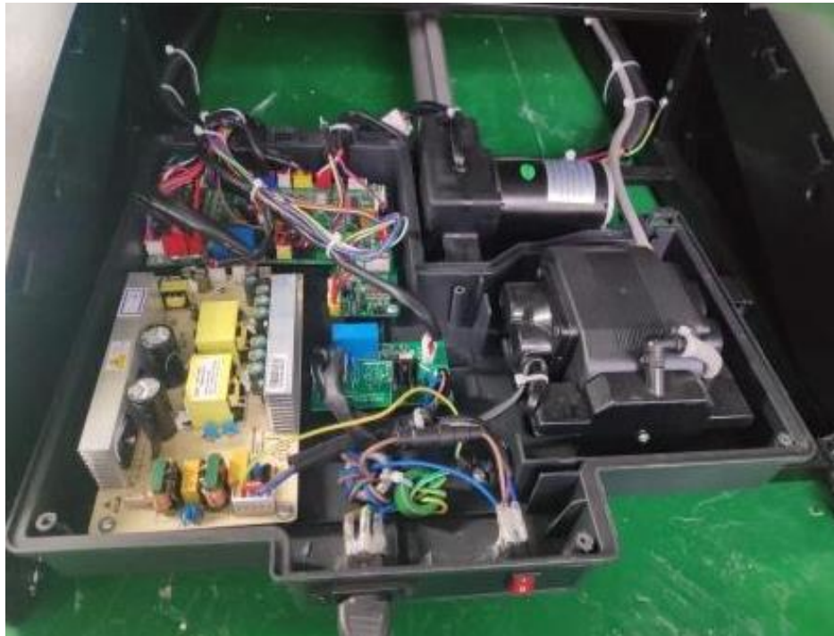
Internal view of centre box
