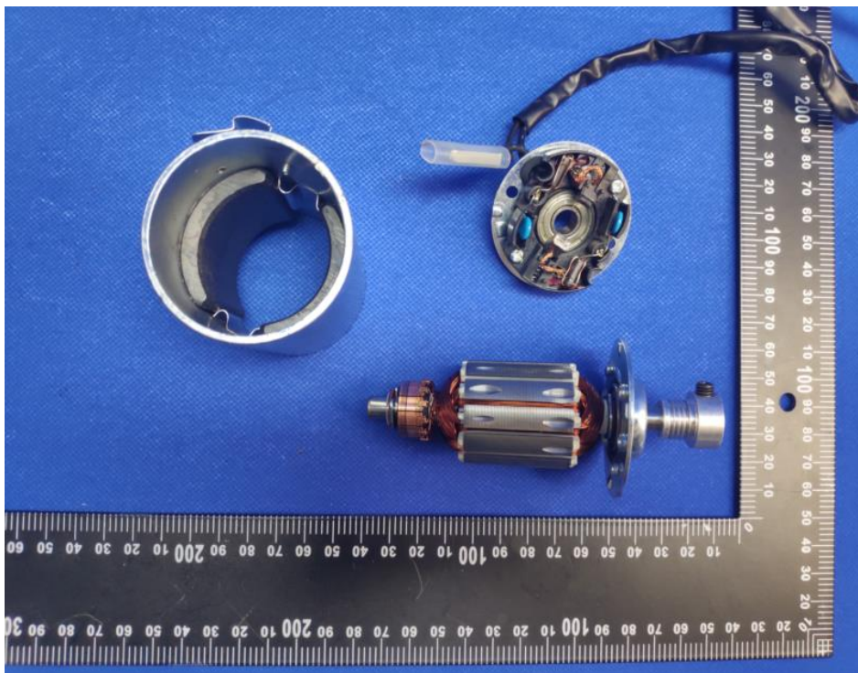
Internal view of tapping motor HS3434D024-G120
