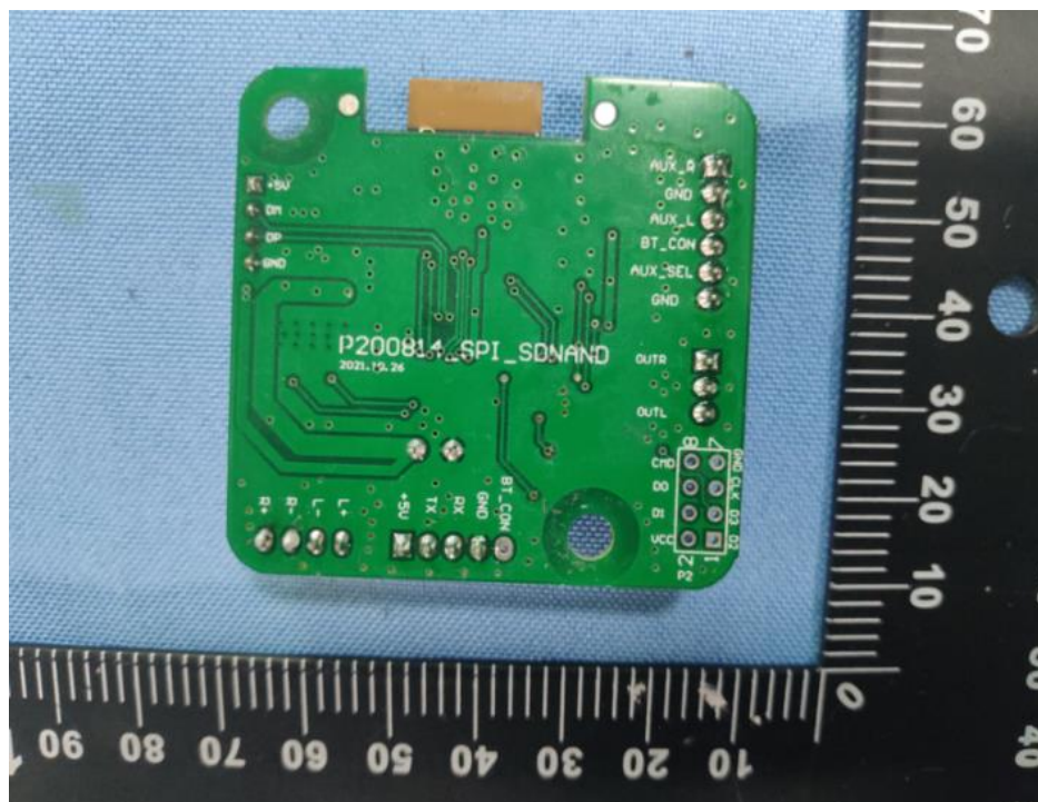
TFT board View
