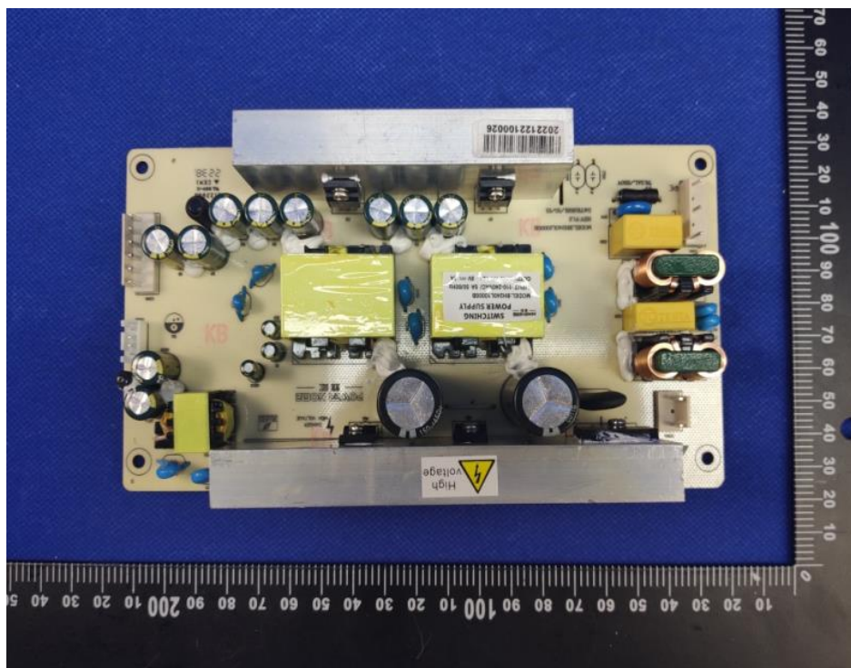
Power PCB View
