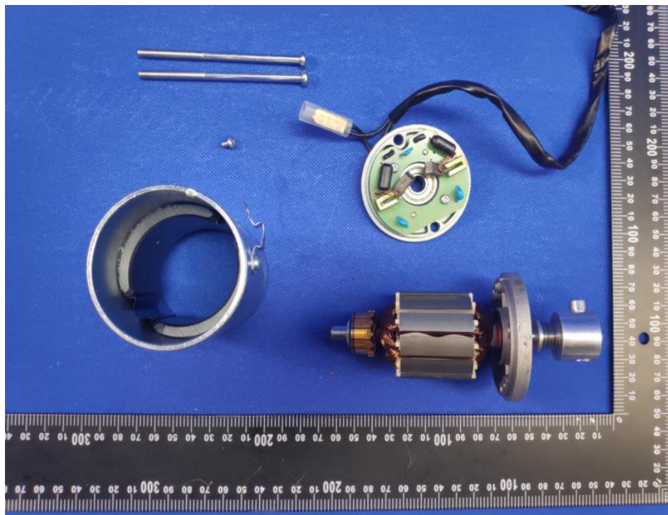
Internal view of Kneading motor HS4435D024-G133
