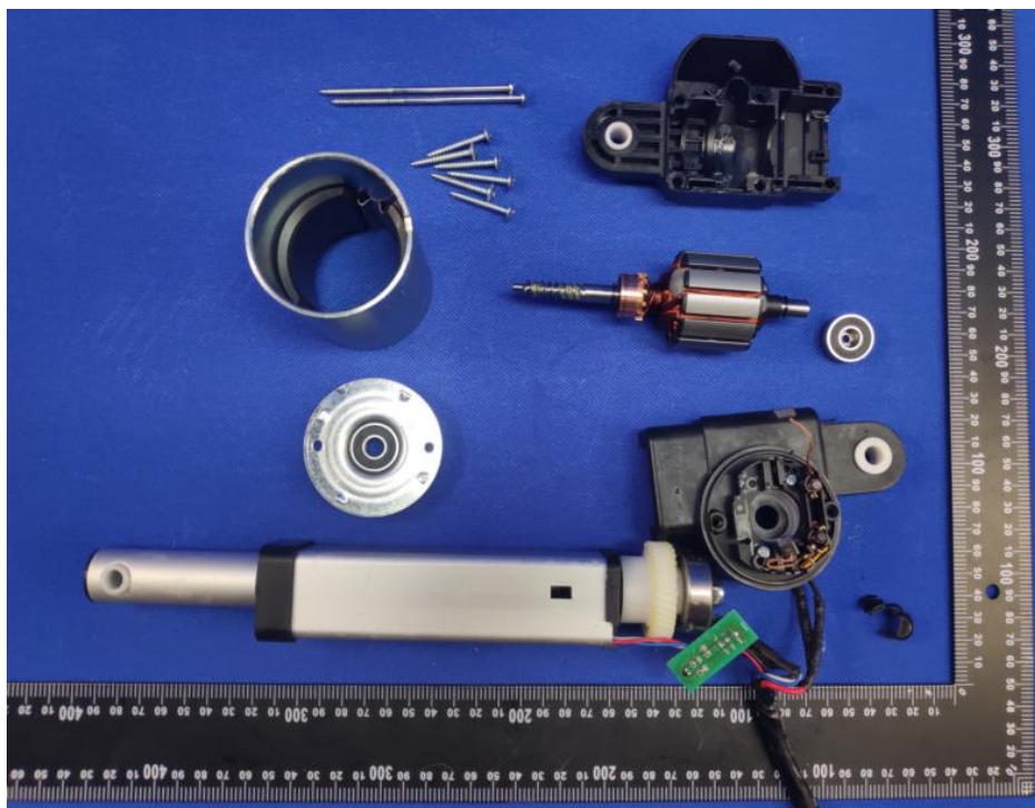
Internal view of Leg adjust motor ZR-252-88JS-HR
