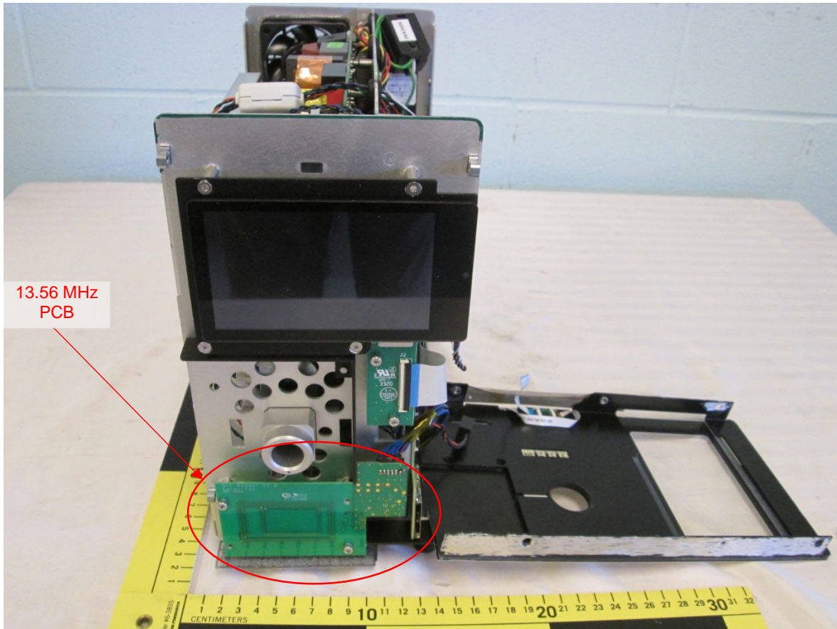
EUT – Internal view 3 Front cover removed 13.56 MHz PCB location indicated
