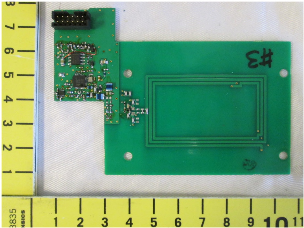
EUT – Internal view 5 Close-up of 13.56 MHz PCB, side 2
