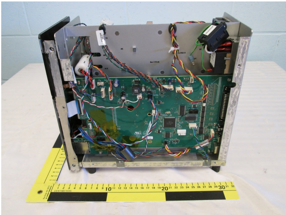
EUT – Internal view 2 Cover removed. EUT left side
