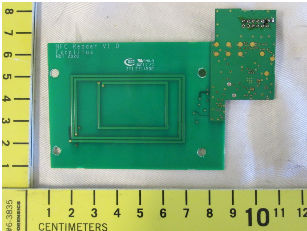
EUT – Internal view 4 Close-up of 13.56 MHz PCB, side 1
