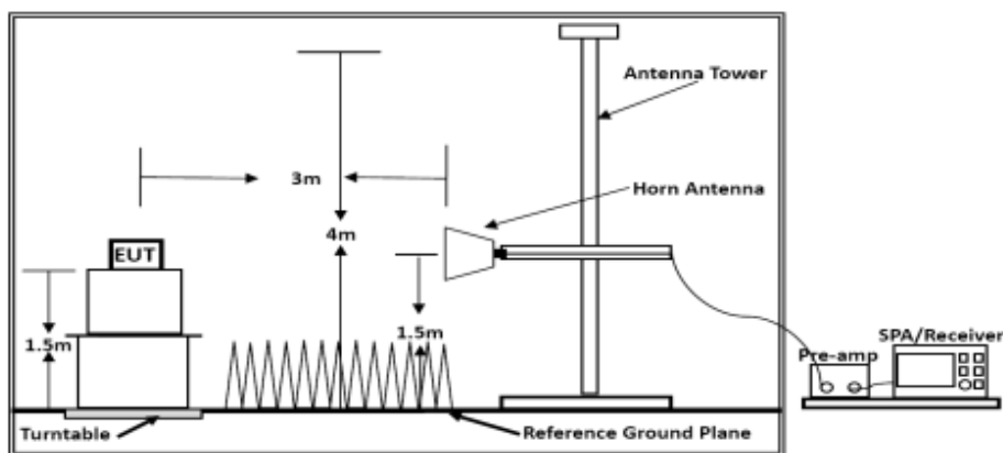
Above 1GHz
