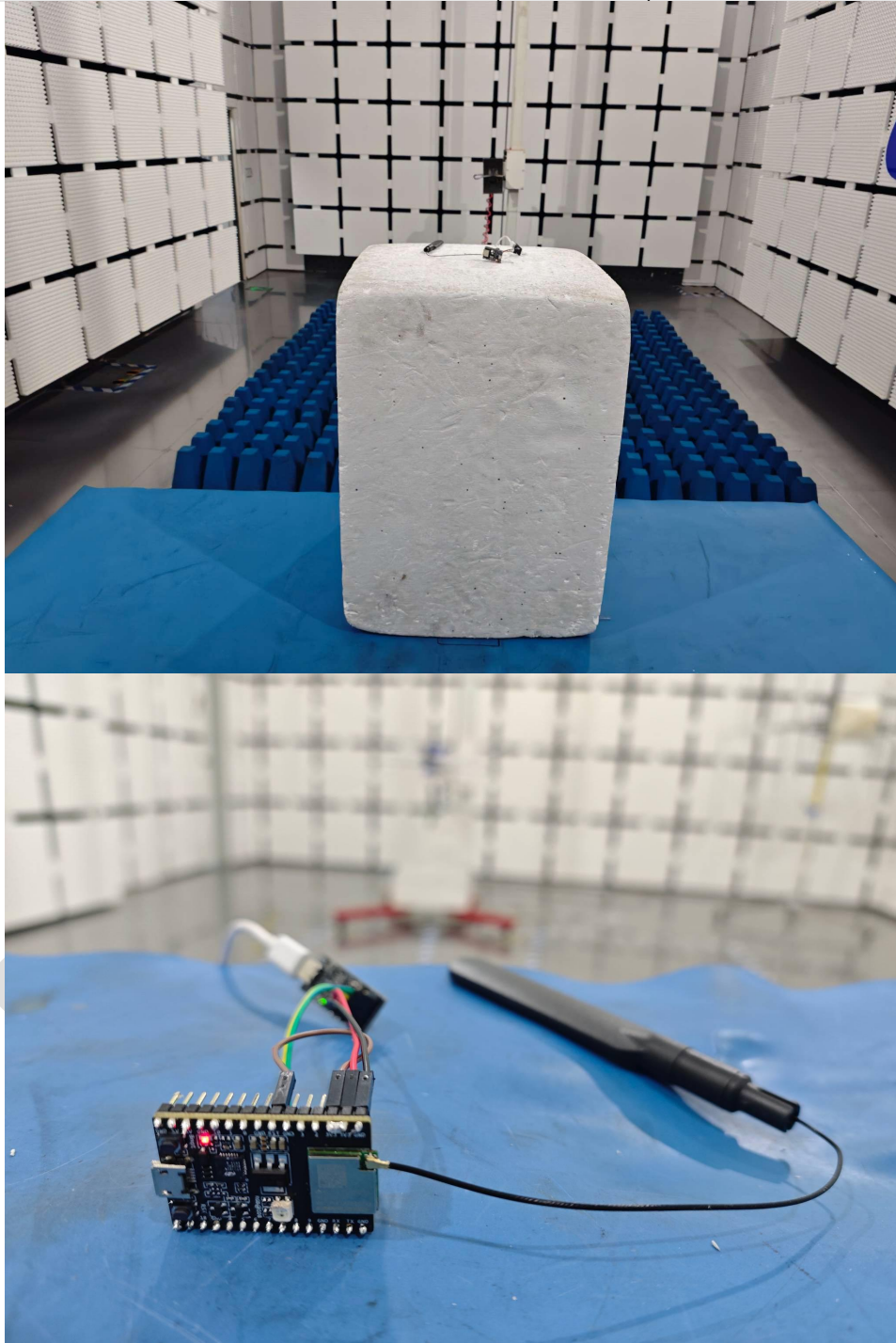
Radiated Emissions (above 1GHz)
