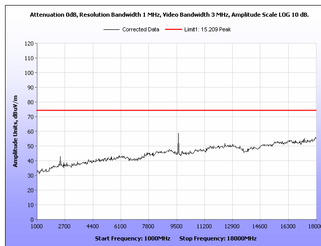
Plot 9: Radiated Spurious Emissions, Low Channel 2405MHz, Peak.
