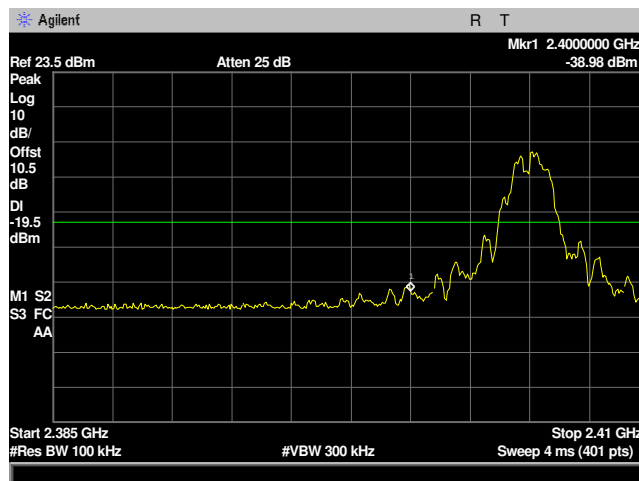
Plot 24: Conducted Spurious Emissions Band Edge 2405MHz Low Channel
