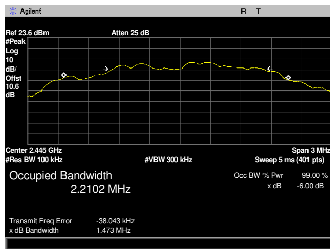
Plot 2: 6dB Occupied Bandwidth 2445MHz Mid Channel
