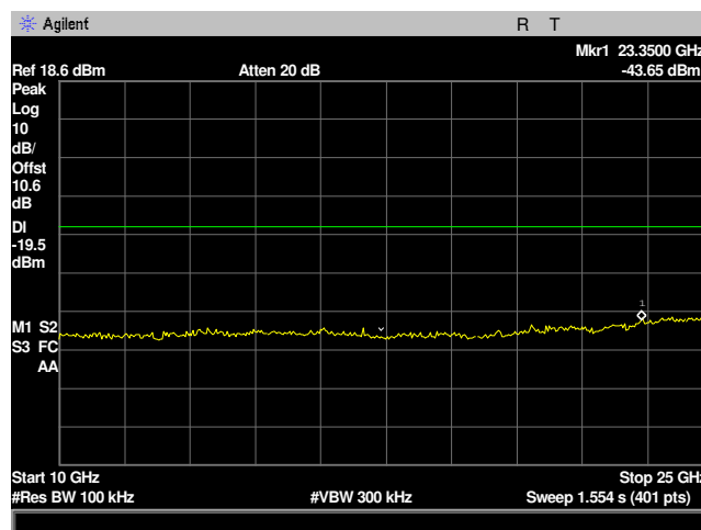
Plot 22: Conducted Spurious Emissions 10GHz-25GHz 2445MHz Mid Channel
