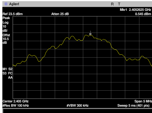
Plot 29: Peak Power Spectral Density 2405MHz Low Channel
