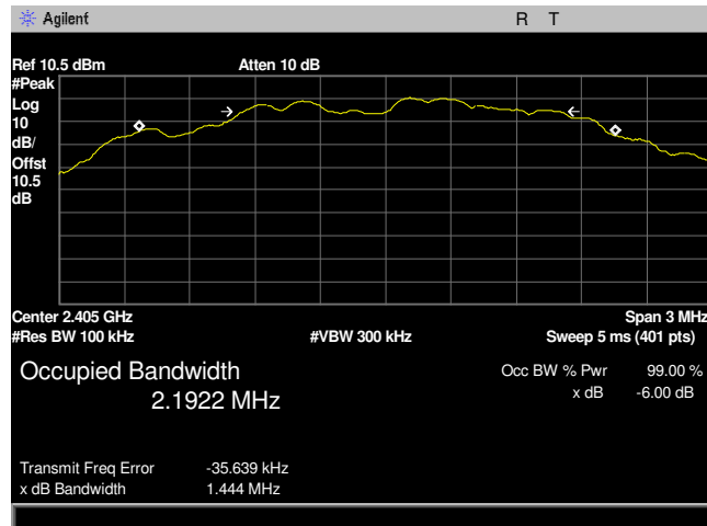
Plot 1: 6dB Occupied Bandwidth 2405MHz Low Channel
