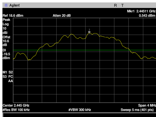
Plot 27: Conducted Spurious Emissions Reference Level 2445MHz Mid Channel
