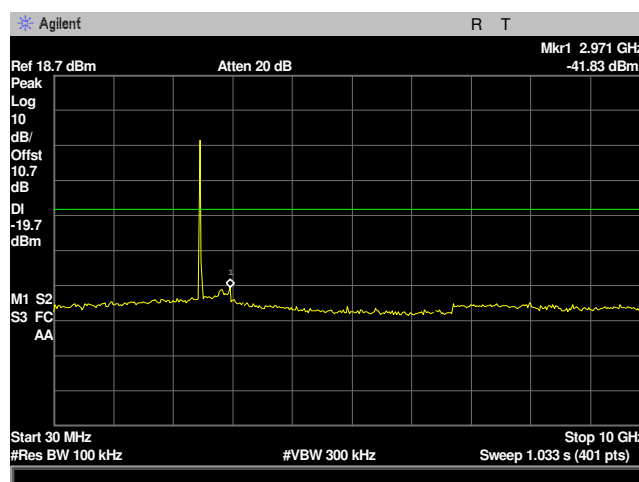
Plot 20: Conducted Spurious Emissions 30MHz-10GHz 2480MHz High Channel
