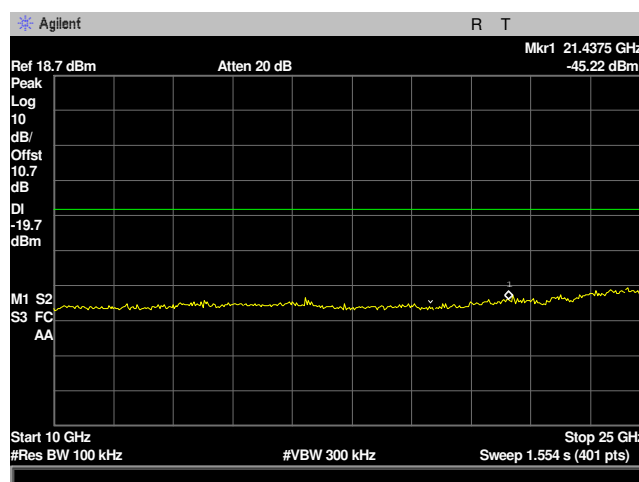
Plot 23: Conducted Spurious Emissions 10GHz-25GHz 2480MHz High Channel
