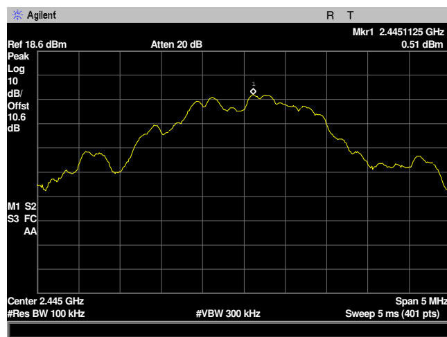
Plot 30: Peak Power Spectral Density 2445MHz Mid Channel
