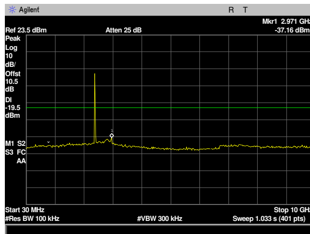
Plot 18: Conducted Spurious Emissions 30MHz-10GHz 2405MHz Low Channel
