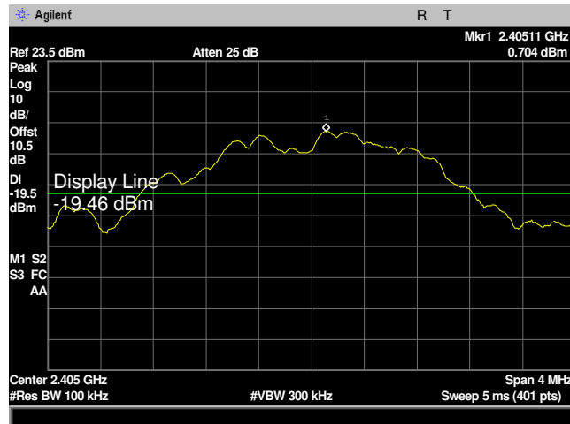
Plot 26: Conducted Spurious Emissions Reference Level 2405MHz Low Channel
