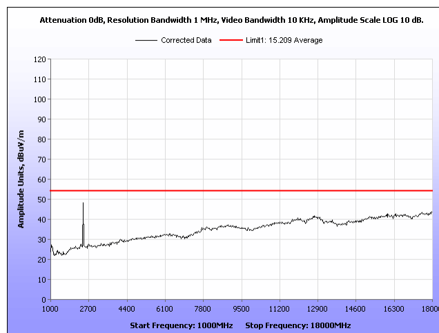
Plot 10: Radiated Spurious Emissions, Mid Channel 2445MHz, Average.
