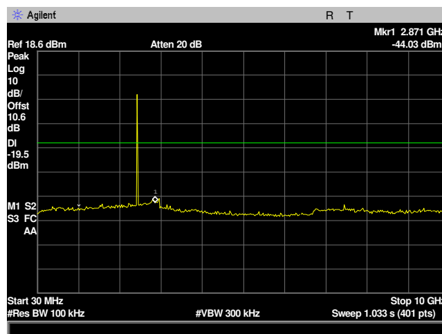
Plot 19: Conducted Spurious Emissions 30MHz-10GHz 2445MHz Mid Channel
