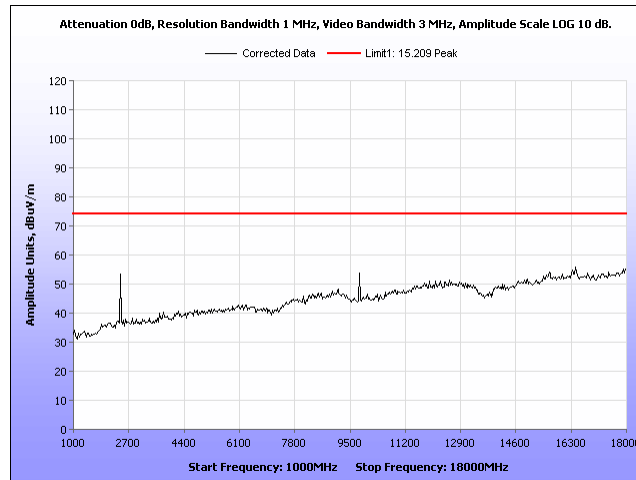
Plot 11: Radiated Spurious Emissions, Mid Channel 2445MHz, Peak.
