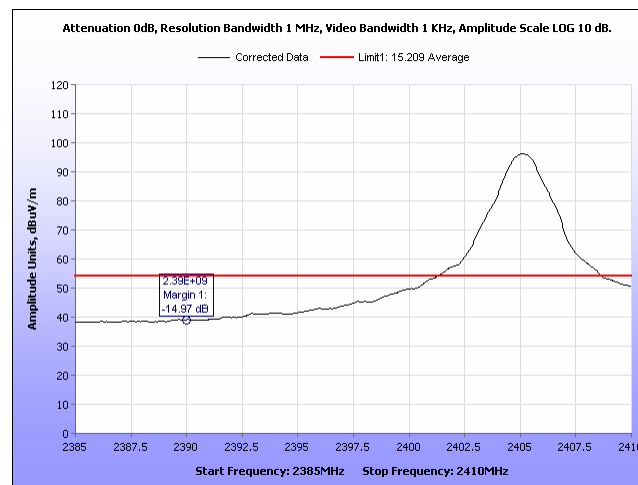
Plot 14: Radiated Band Edge, Low Channel 2405MHz, Average.
