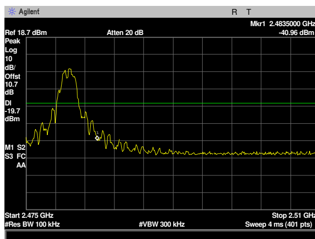
Plot 25: Conducted Spurious Emissions Band Edge 2480MHz High Channel
