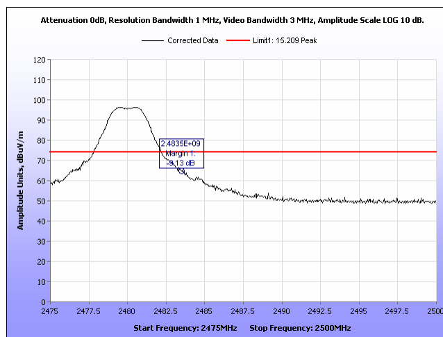
Plot 17 Radiated Band Edge, High Channel 2480MHz, Peak.
