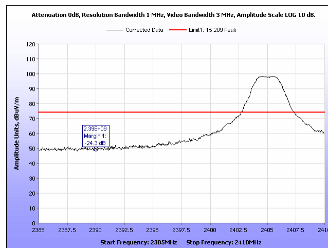
Plot 15: Radiated Band Edge, Low Channel 2405MHz, Peak.
