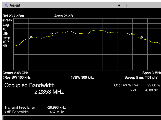
Plot 3: 6dB Occupied Bandwidth 2480MHz High Channel
