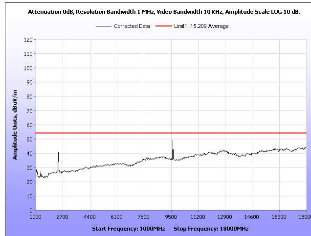
Plot 8: Radiated Spurious Emissions, Low Channel 2405MHz, Average.
