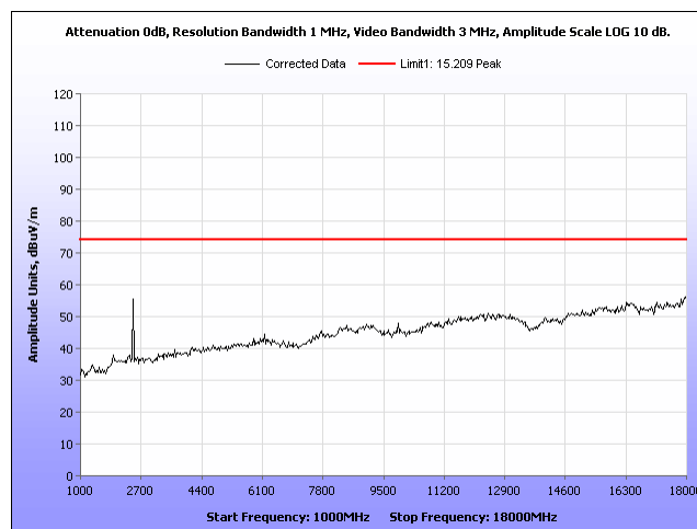
Plot 13 Radiated Spurious Emissions, High Channel 2480MHz, Peak.
