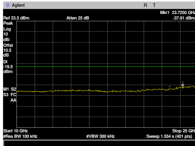
Plot 21: Conducted Spurious Emissions 10GHz-25GHz 2405MHz Low Channel
