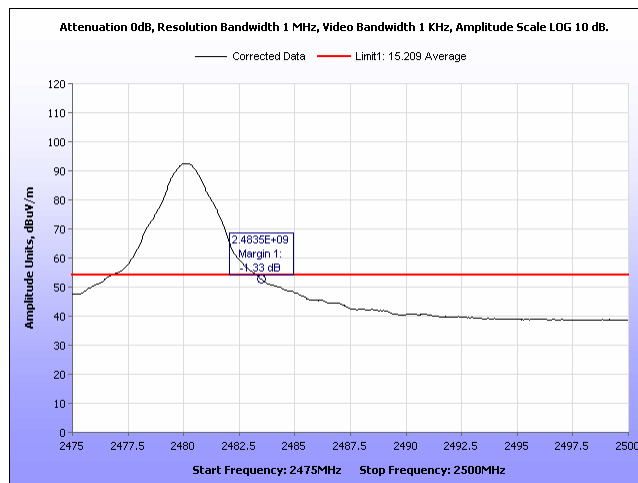
Plot 16: Radiated Band Edge, High Channel 2480MHz, Average.
