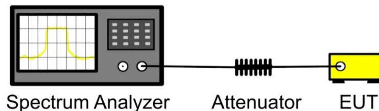
Figure 1: Occupied Bandwidth Test Setup
