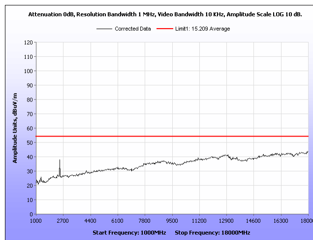
Plot 12: Radiated Spurious Emissions, High Channel 2480MHz, Average.
