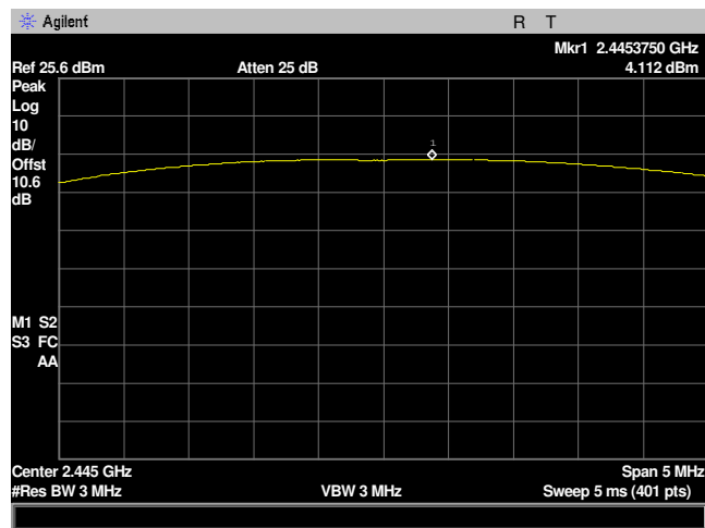
Plot 5: Peak Power Output 2445MHz Mid Channel
