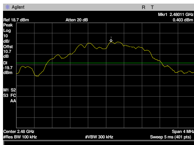
Plot 28: Conducted Spurious Emissions Reference Level 2480MHz High Channel
