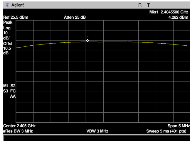
Plot 4: Peak Power Output 2405MHz Low Channel
