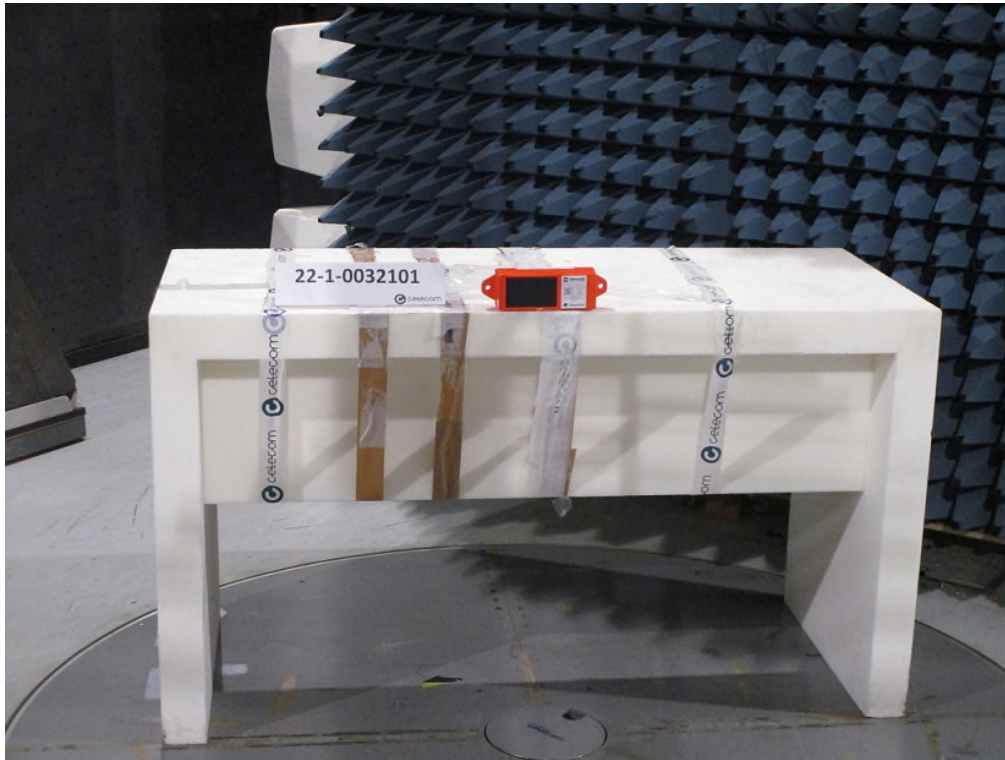
Fig. Mea.: 1 : Radiated Emission Picture1
