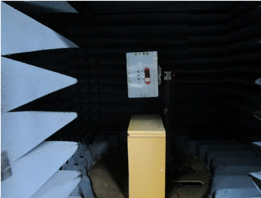
Fig. Mea.: 3 : Radiated Emission above 1GHz, Picture3
