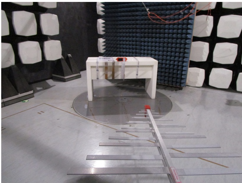
Fig. Mea.: 2 : Radiated Emission Picture1
