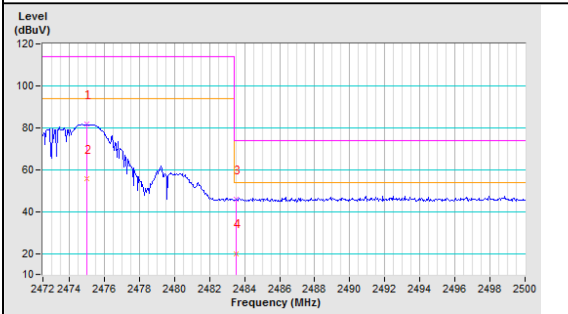
2475MHz Vertical
