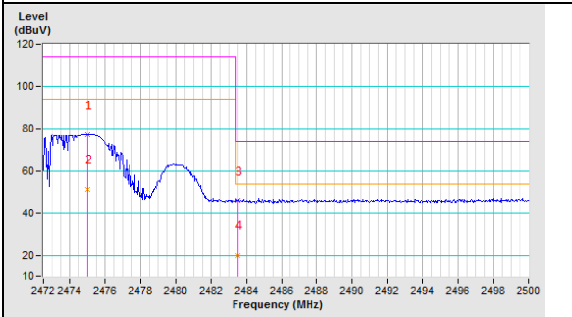
2475MHz Vertical
