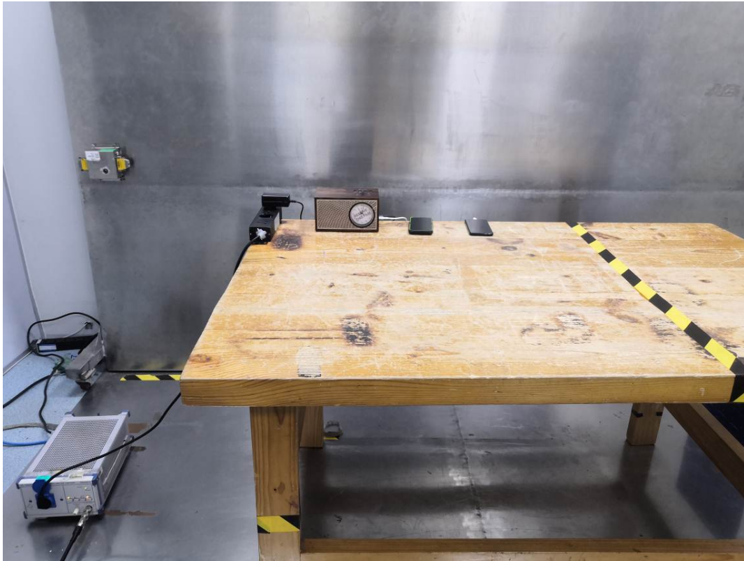
Conducted Emissions Side View –Model: DESSBX
