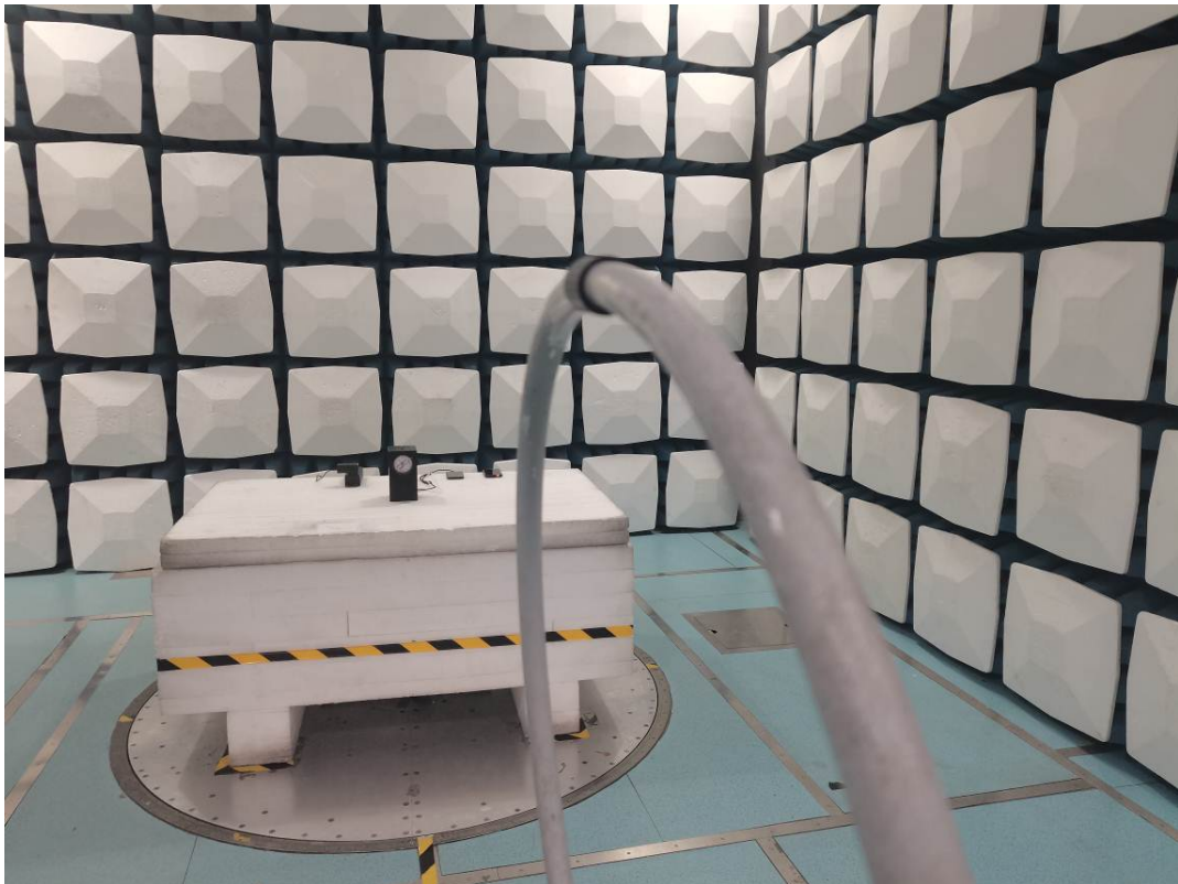
Radiated Emission 9k-30MHz Perpendicular View-Model: UBSSBX
