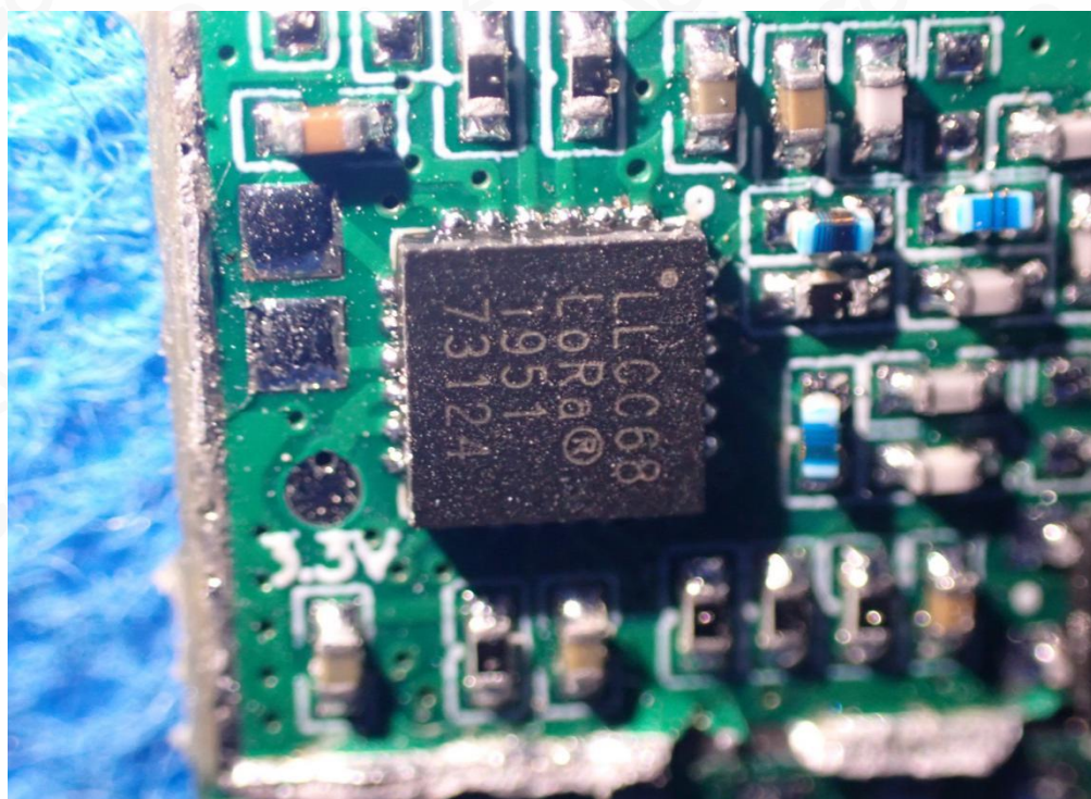
INTERNAL VIEW-2 OF EUT
