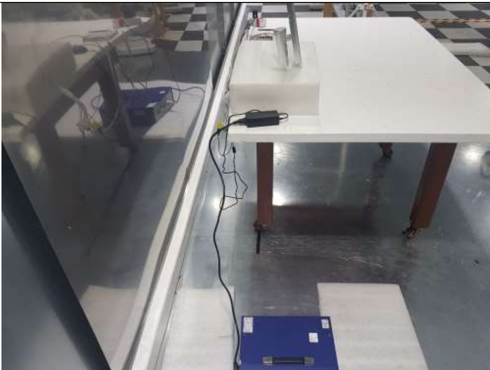
AC Power Line Conducted Emission 2
