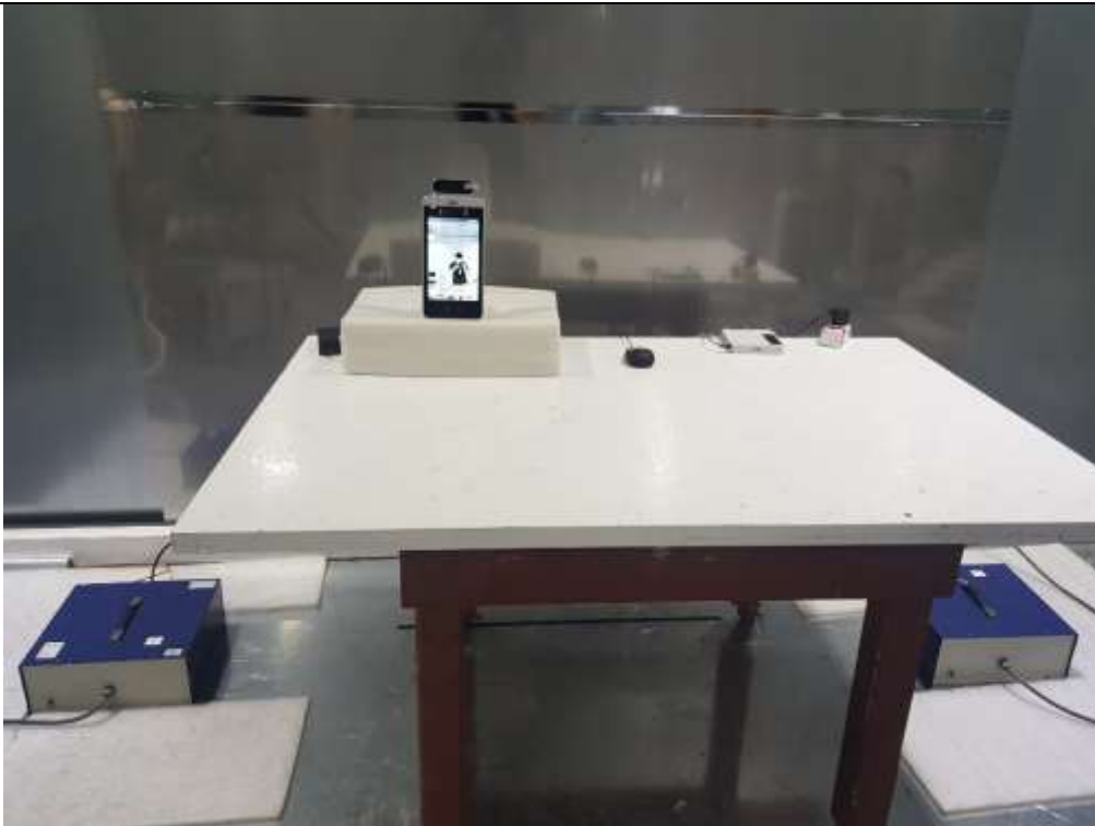
AC Power Line Conducted Emission 1
