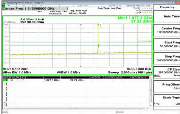
30MHz~3GHz_Band2_5MHz_QPSK_1_0_MidCH18900-1880
