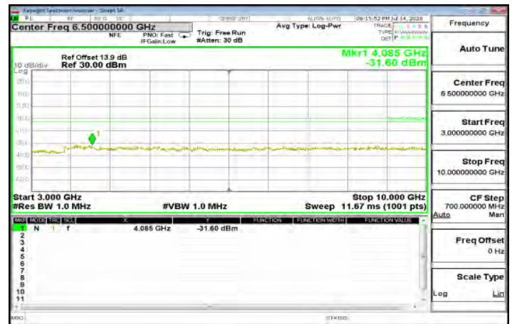
Spurious Emission High_ HSUPA_B5_Mid CH4183-836.6
