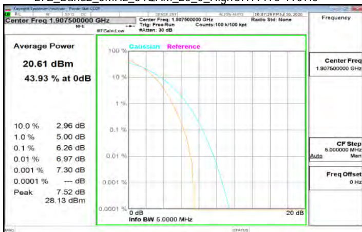
LTE_Band2_5MHz_64QAM_25_0_HighCH19175-1907.5
