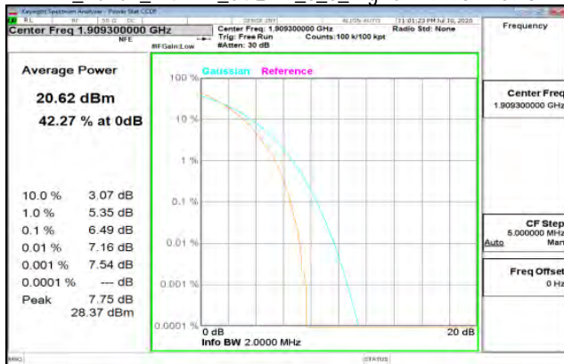
LTE_Band2_1.4MHz_64QAM_6_0_HighCH19193-1909.3
