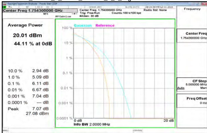
LTE_Band4_1_4MHz_64QAM_6_0_HighCH20393-1754.3
