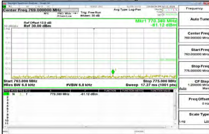
Inband-2_Band13_5MHz_QPSK_1_0_HighCH23255-784.5
