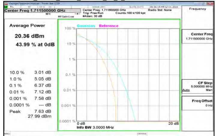
LTE_Band4_3MHz_64QAM_15_0_LowCH19965-1711.5
