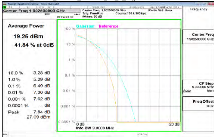
LTE_Band2_15MHz_64QAM_75_0_HighCH19125-1902.5
