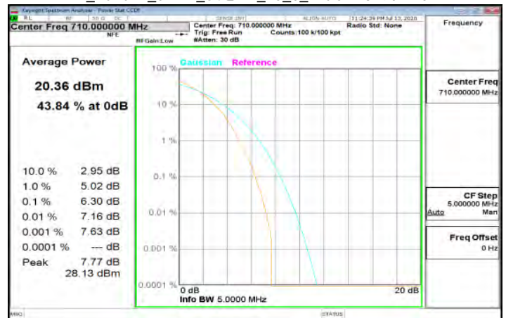
LTE_Band17_5MHz_64QAM_25_0_MidCH23790-710
