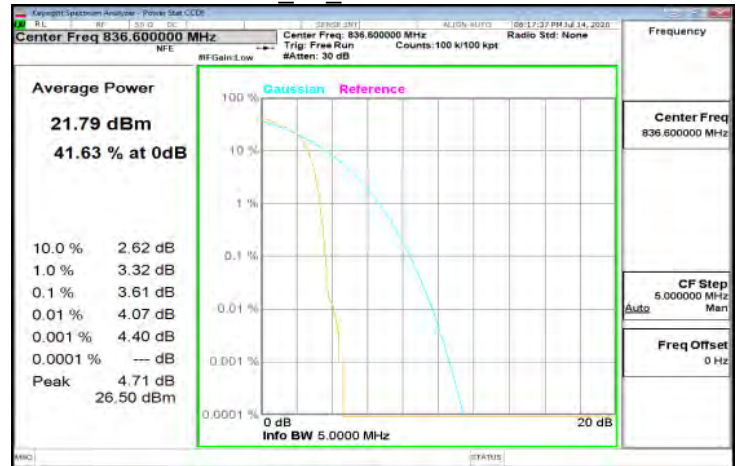
HSUPA B5 MidCH4183-836.6
