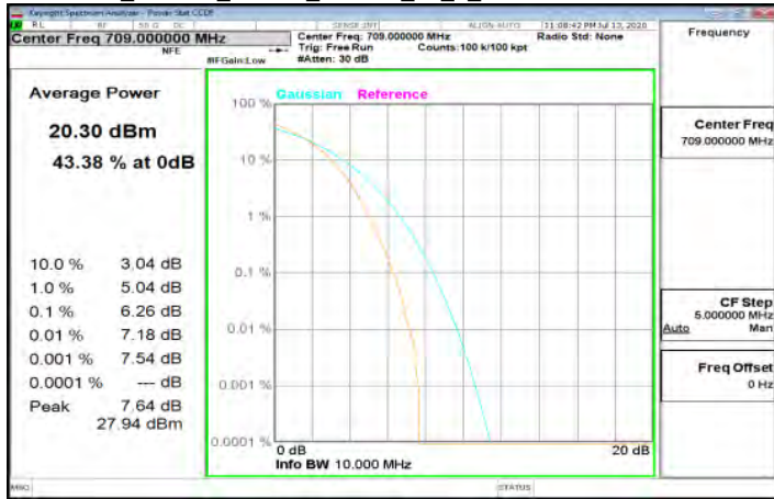
LTE_Band17_10MHz_64QAM_50_0_MidCH23790-710
