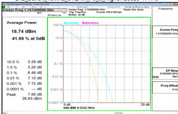
LTE_Band4_15MHz_64QAM_75_0_HighCH20325-1747.5
