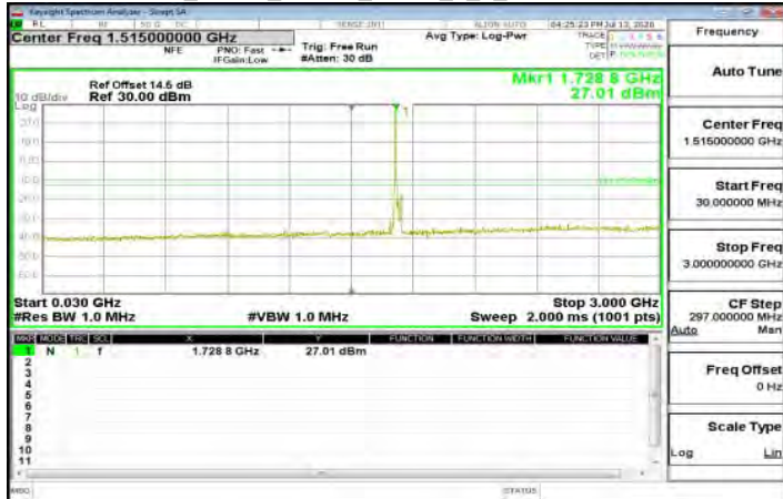
30MHz~3GHz_Band4_15MHz_QPSK_1_0_MidCH20175-1732.5
