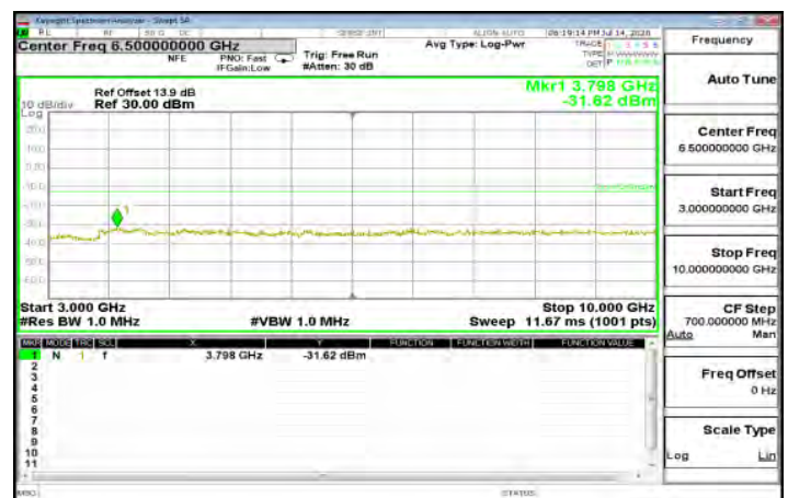
Spurious Emission High_ HSUPA_B5_HighCH4233-846.6
