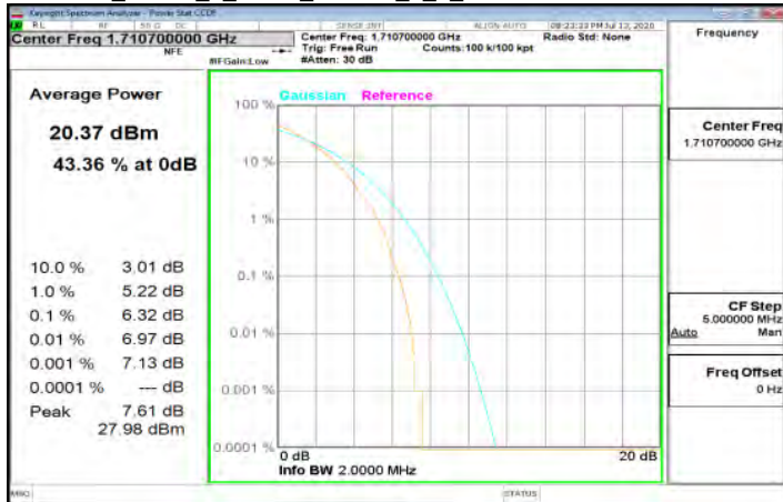
LTE_Band4_1_4MHz_64QAM_6_0_LowCH19957-1710.7
