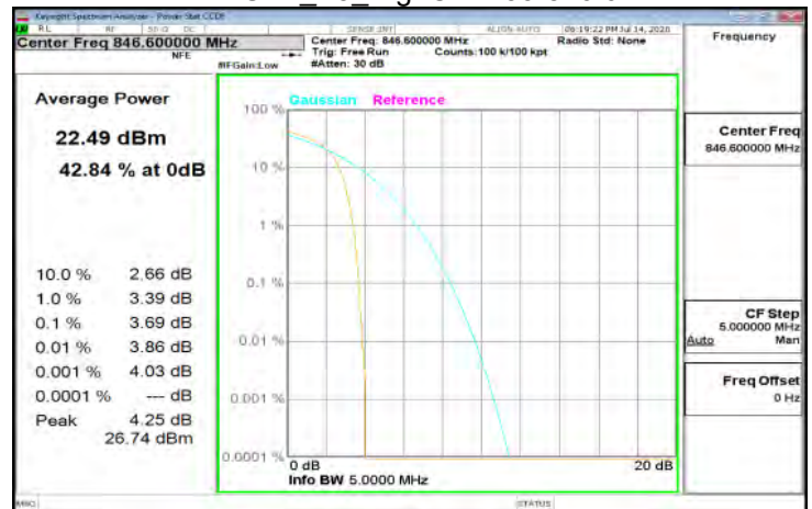
HSUPA B5 HighCH4233-846.6
