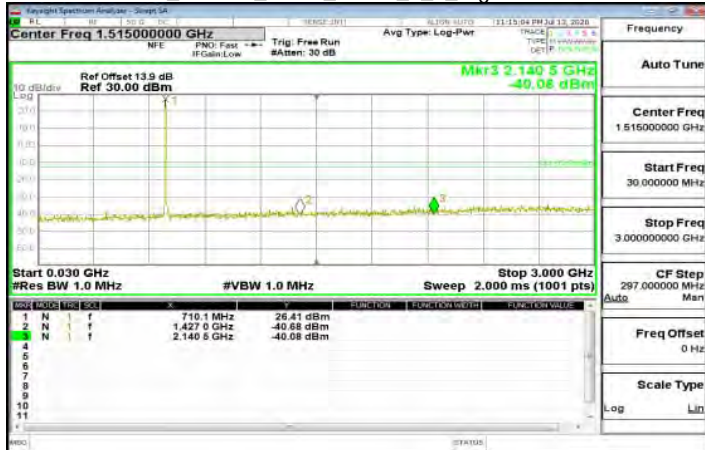
30MHz~3GHz_Band17_5MHz_QPSK_1_0_HighCH23825-713.5
