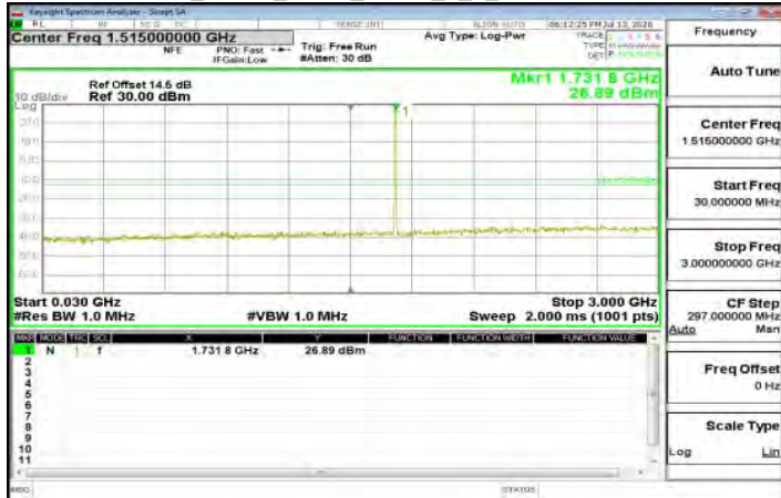
30MHz-3GHz_Band4_3MHz_QPSK_1_0_MidCH20175-1732.5
