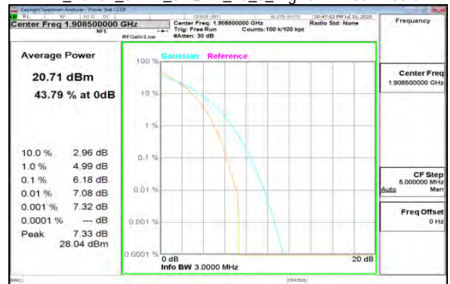
LTE_Band2_3MHz_64QAM_15_0_HighCH19185-1908.5
