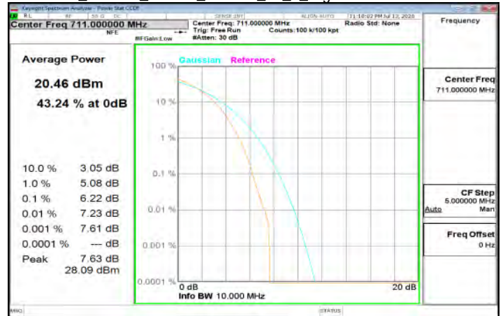
LTE_Band17_10MHz_64QAM_50_0_HighCH23800-711
