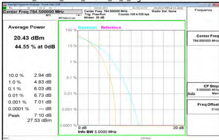
LTE_Band13_5MHz_64QAM_25_0_HighCH23255-784.5
