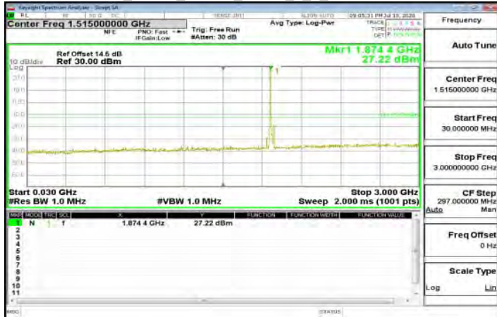
30MHz~3GHz_Band2_15MHz_QPSK_1_0_MidCH18900-1880
