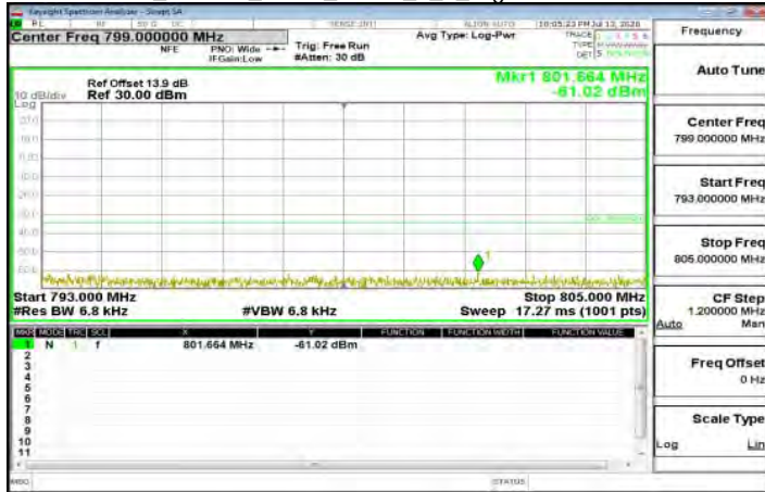
Inband-1_Band13_10MHz_QPSK_1_0_MidCH23230-782
