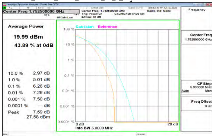
LTE_Band4_5MHz_64QAM_25_0_HighCH20375-1752.5
