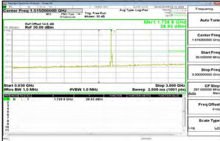
30MHz~3GHz_Band4_10MHz_QPSK_1_0_MidCH20175-1732.5
