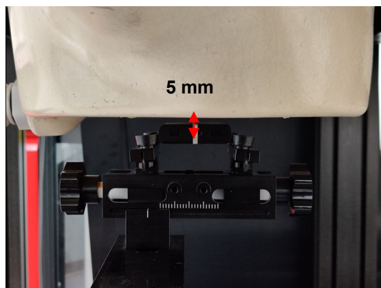
Photograph 12. Body-worn, Front Surface, 5mm
