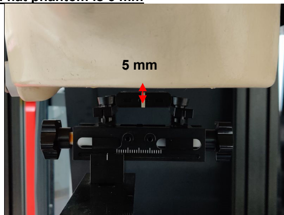
Photograph 10. Body-worn, Back Surface, 5mm
