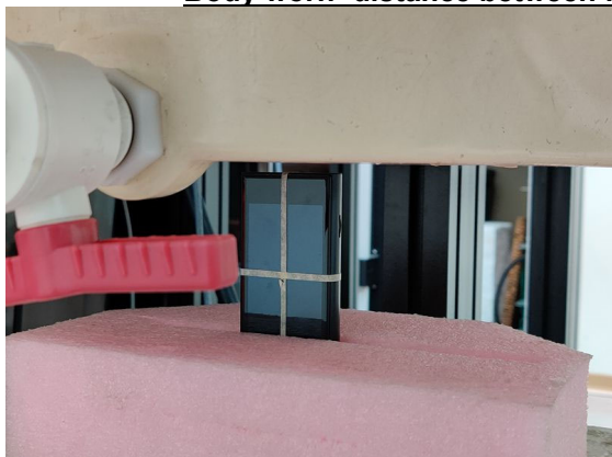
Photograph 15. Body-worn, Bottom Edge, 5mm
