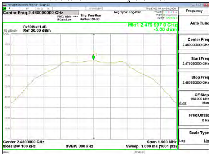
Reference Level_BLE_1M_HighCH39-2480
