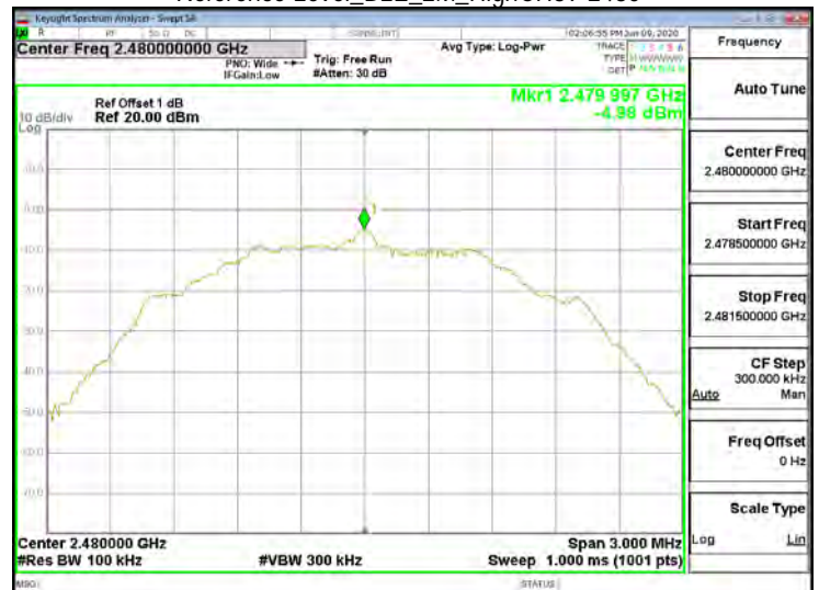
Reference Level_BLE_2M_HighCH39-2480
