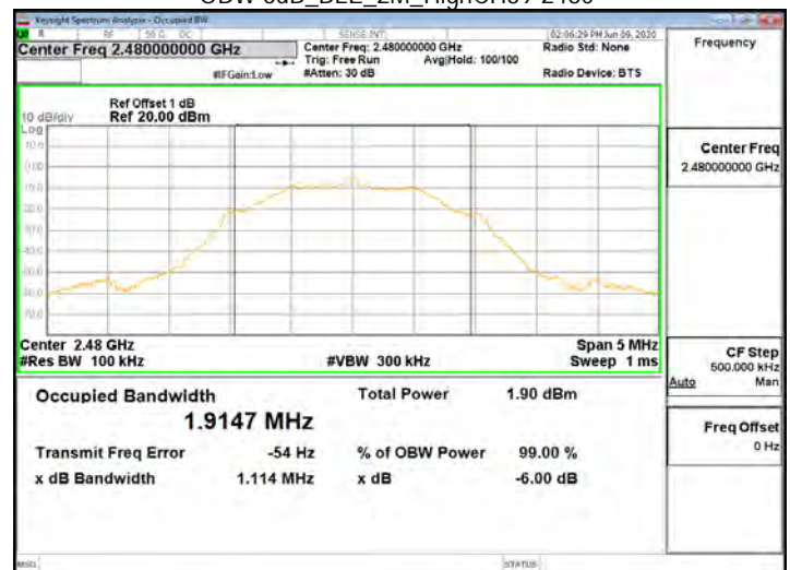
OBW 6dB_BLE_2M_HighCH39-2480
