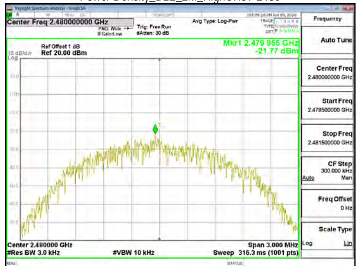
Power Density_BLE_2M_HighCH39-2480
