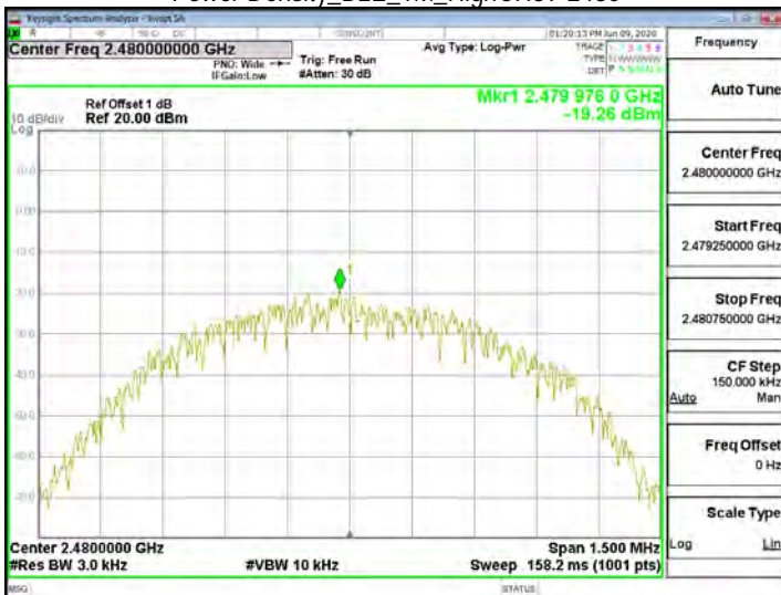
Power Density_BLE_1M_HighCH39-2480
