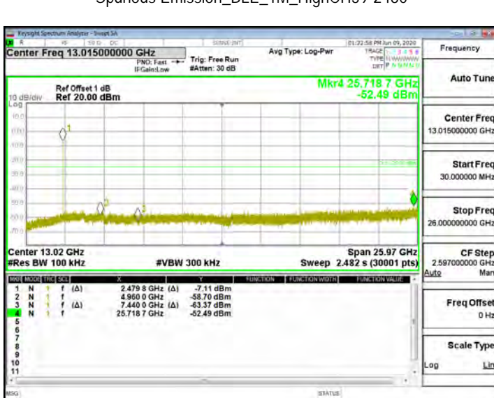
Spurious Emission_BLE_1M_HighCH39-2480
