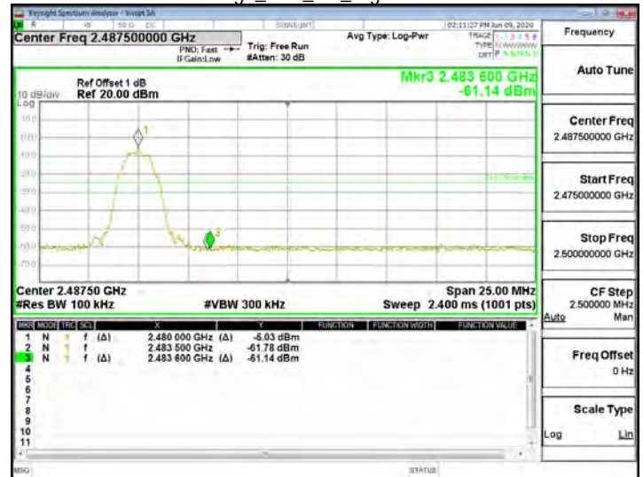
Band Edge_BLE_2M_HighCH39-2480
