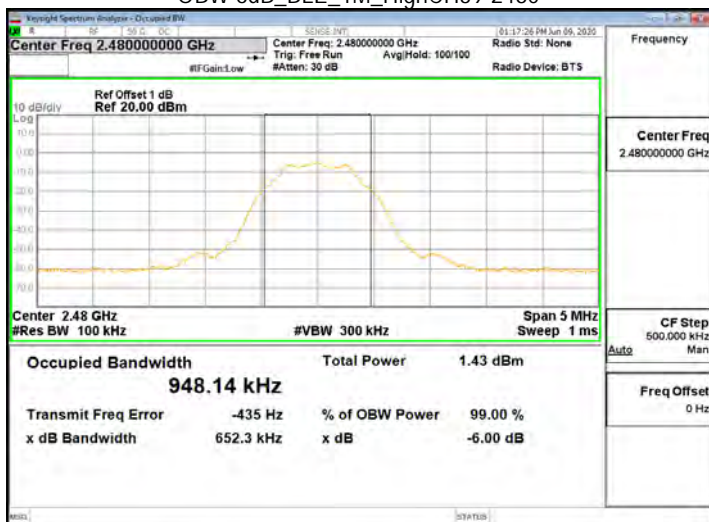
OBW 6dB_BLE_1M_HighCH39-2480
