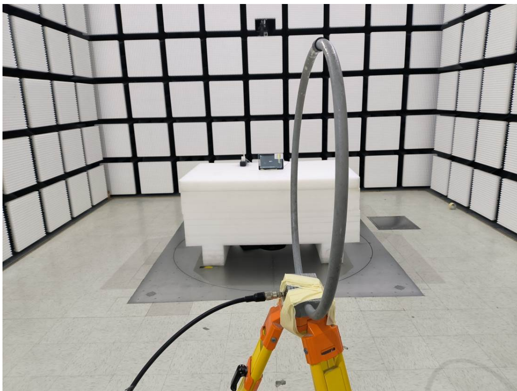
Radiated Emissions 9k-30MHz Perpendicular View #2
