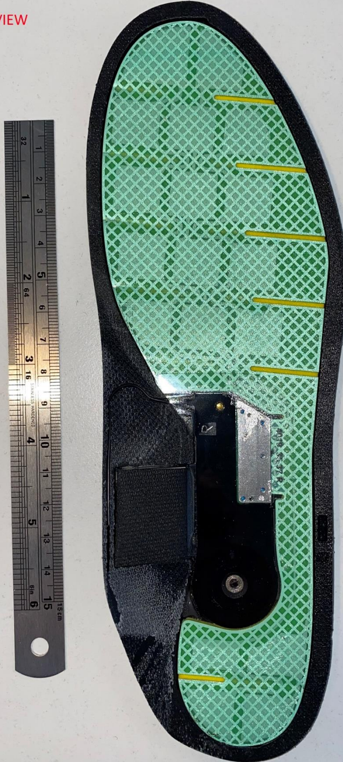
Right insole - Device open view
