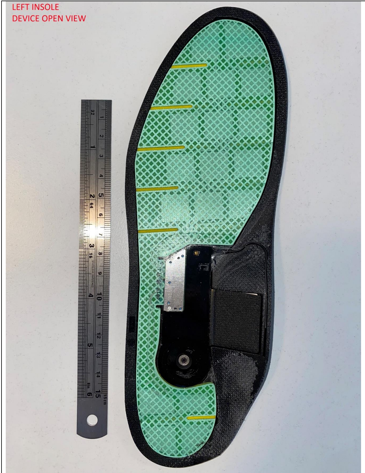
Left insole - Device open view
