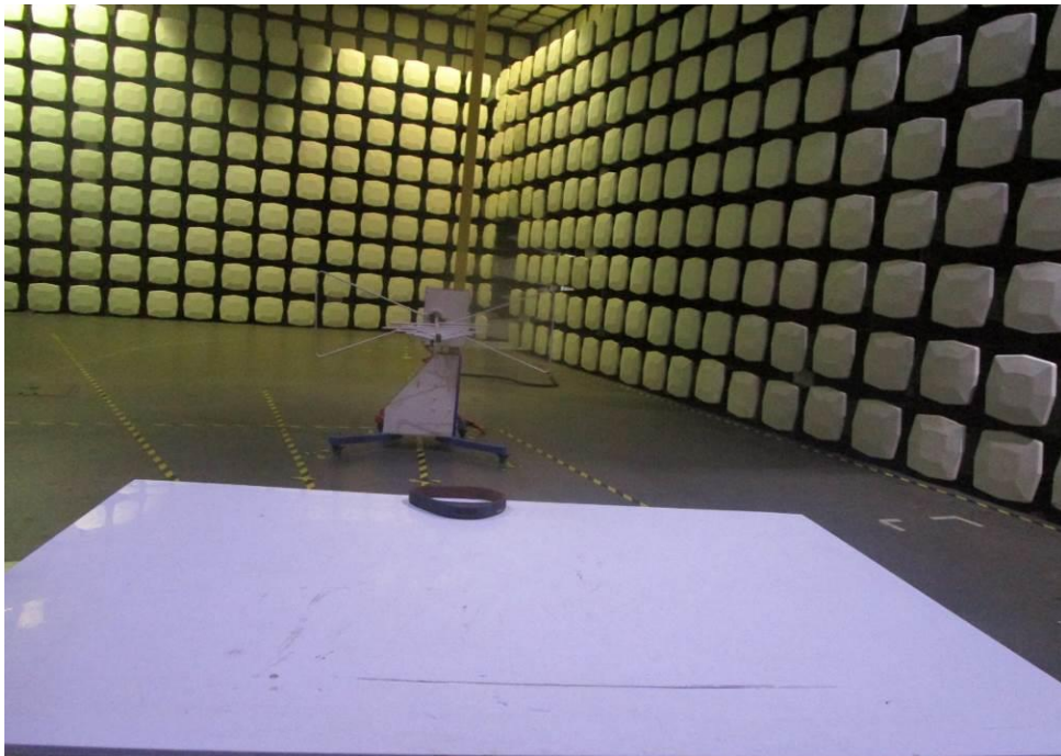
Radiated Spurious Emissions (Below 1GHz)
