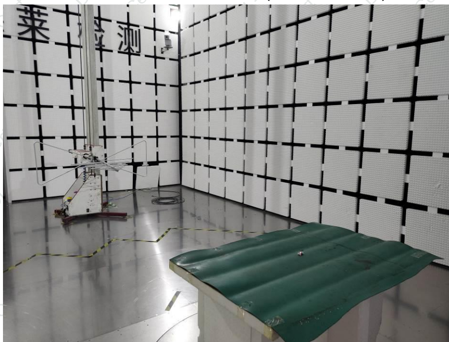
Radiated Measurement Photos ( 30MHz-1000MHz )
