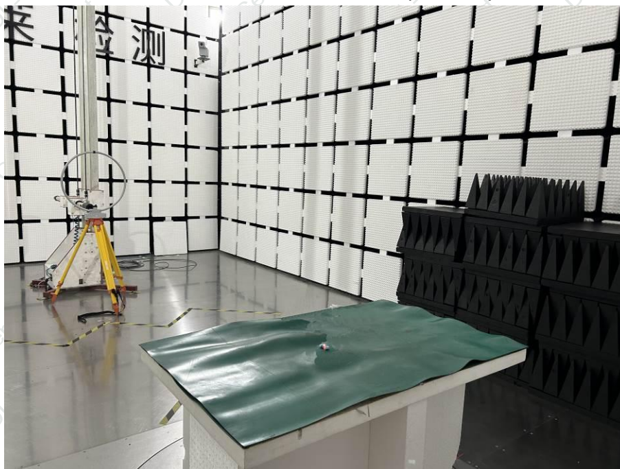
Radiated Measurement Photos ( 9K-30M )
