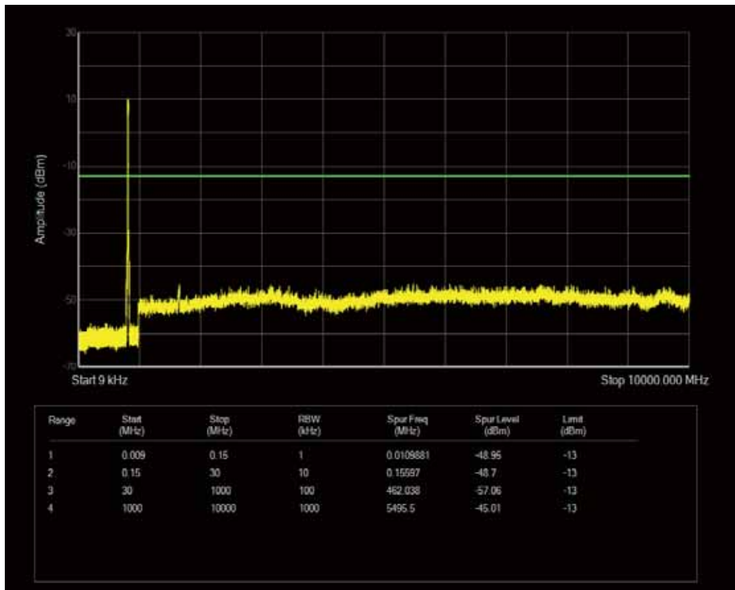
Band26b QAM16 BW=15MHz Channel=26865 RB Size=75 Position=#0
