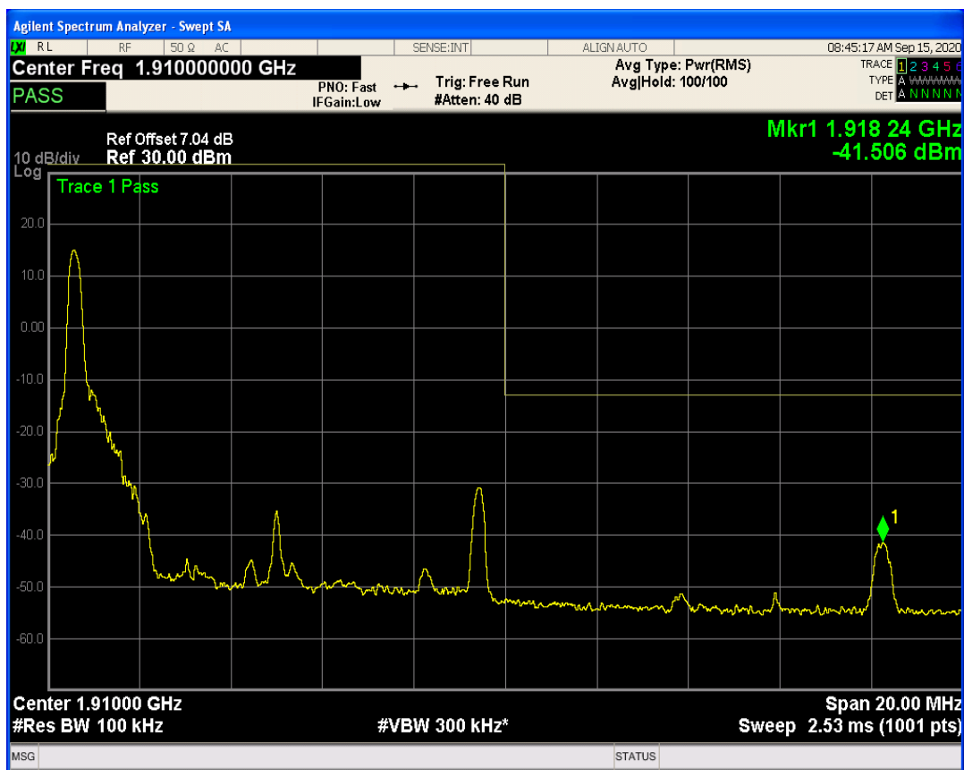
LTE Band2 QPSK BW=10MHz Channel=19150 RB Size=1 Position=#Max
