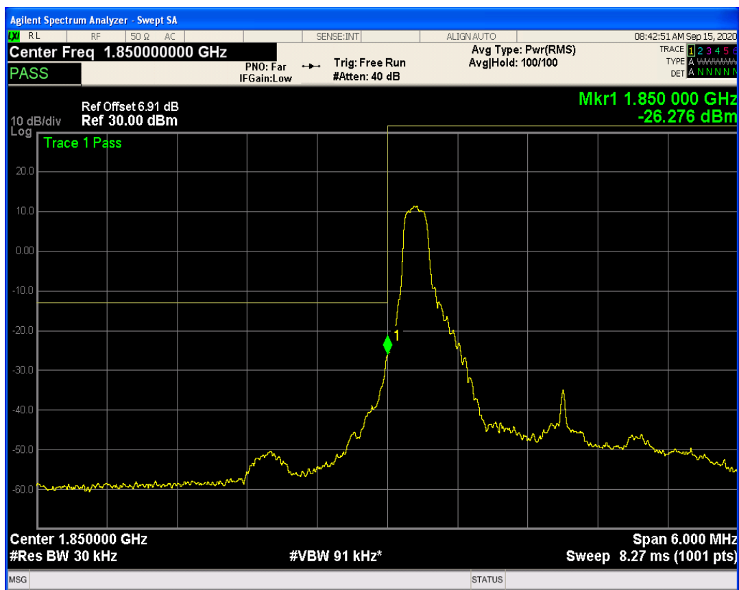
LTE Band2 QPSK BW=3MHz Channel=18615 RB Size=1 Position=#Max
