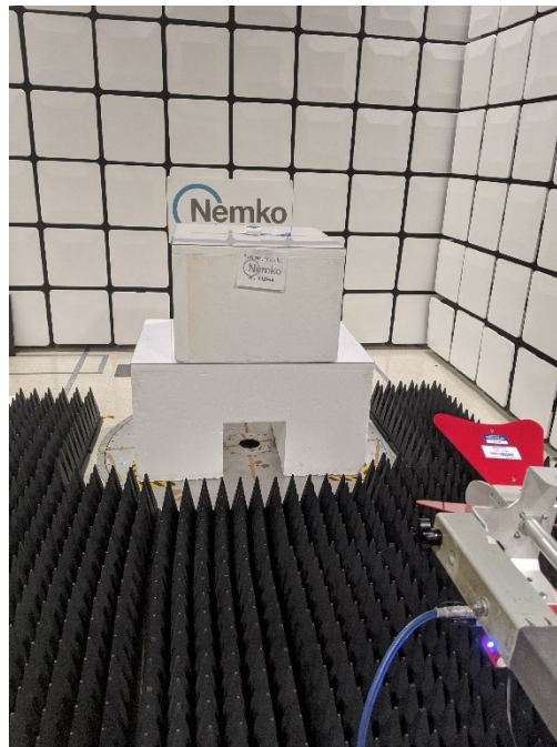
Figure 3 - Radiated emissions above 1 GHz, front view
