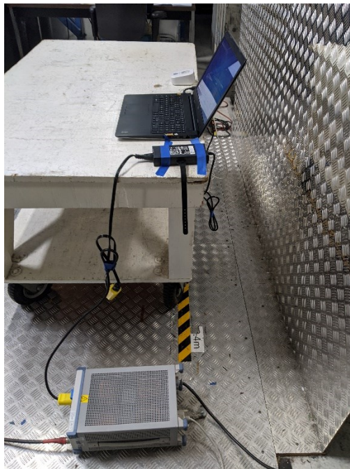
Figure 6 – AC conducted emissions, side view
