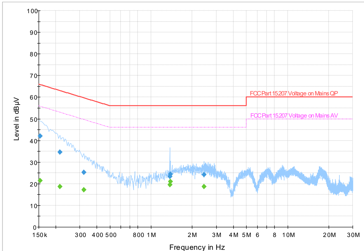
Figure 8.5-1: AC conducted emissions
