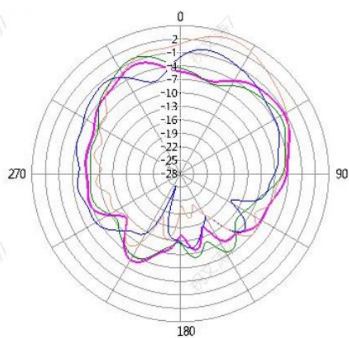
Phi=0 deg
