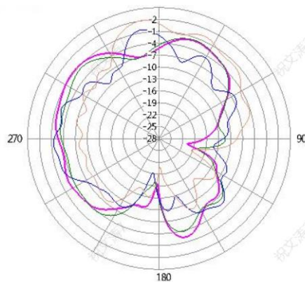
Phi=90 deg
