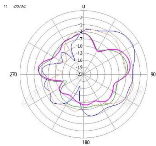
Phi=90 deg
