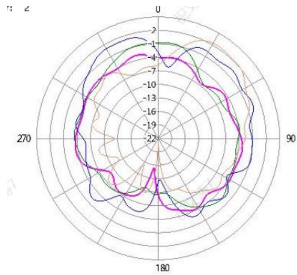
Phi=0 deg
